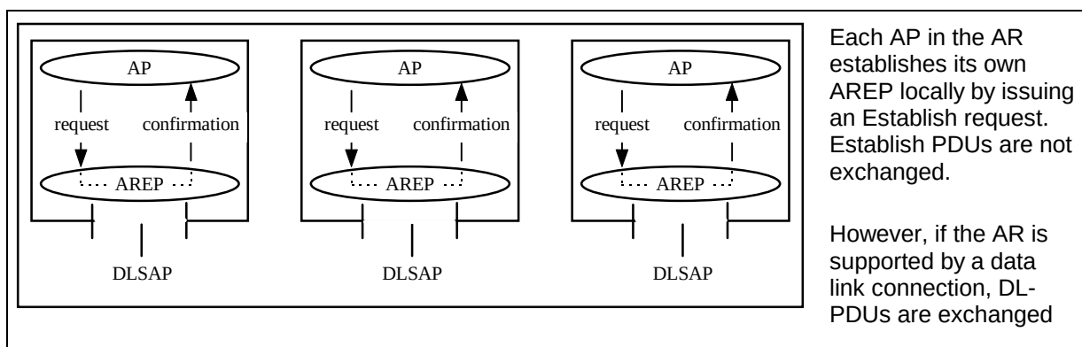
Figure 17 – 1-to-many AR establishment
