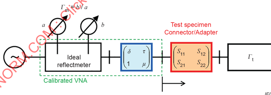
Figure 3 – VNA measurement model
