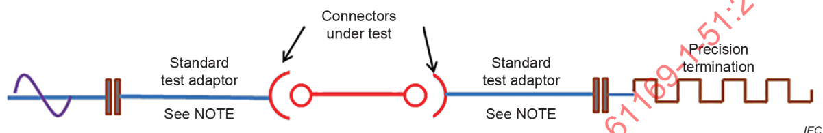
Figure 2 – Graphical principle
