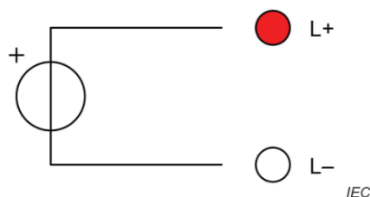
Figure 2 – Colour identification of conductors in DC circuits
