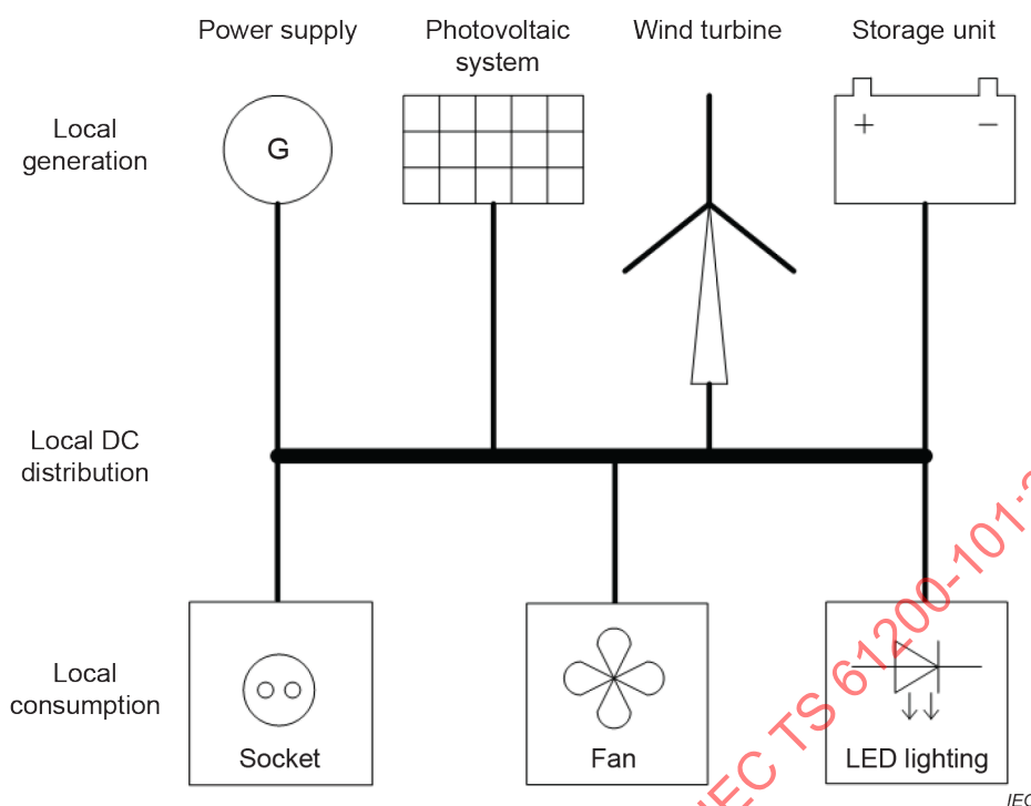
Figure 1 – Concept of a low voltage electrical installation
