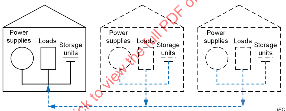
Figure A.4 – DC electrical installation in direct feeding mode
