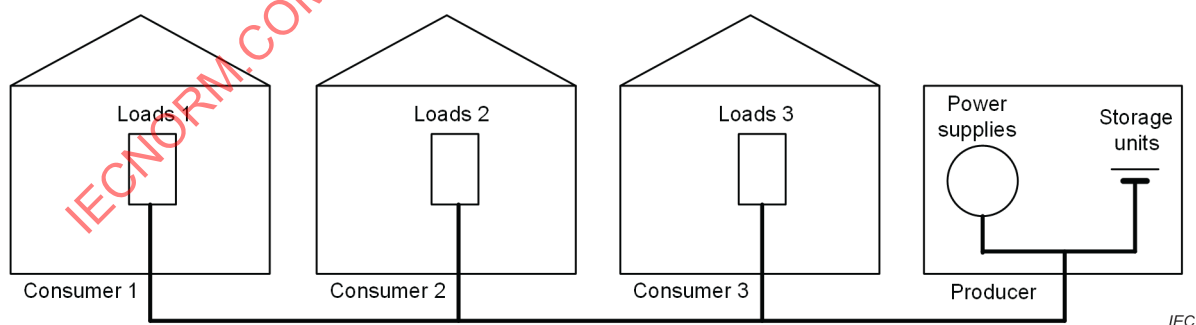
Figure A.2 – Example of a collective installation
