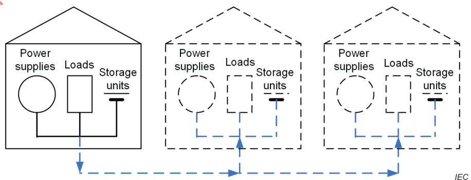
Figure A.5 – DC electrical installation in reverse feeding mode
