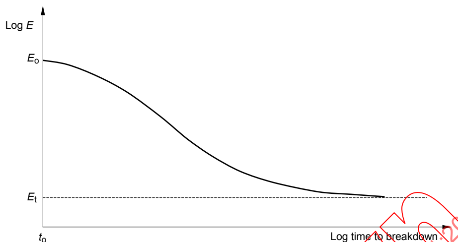
Figure 1 – General voltage endurance line
