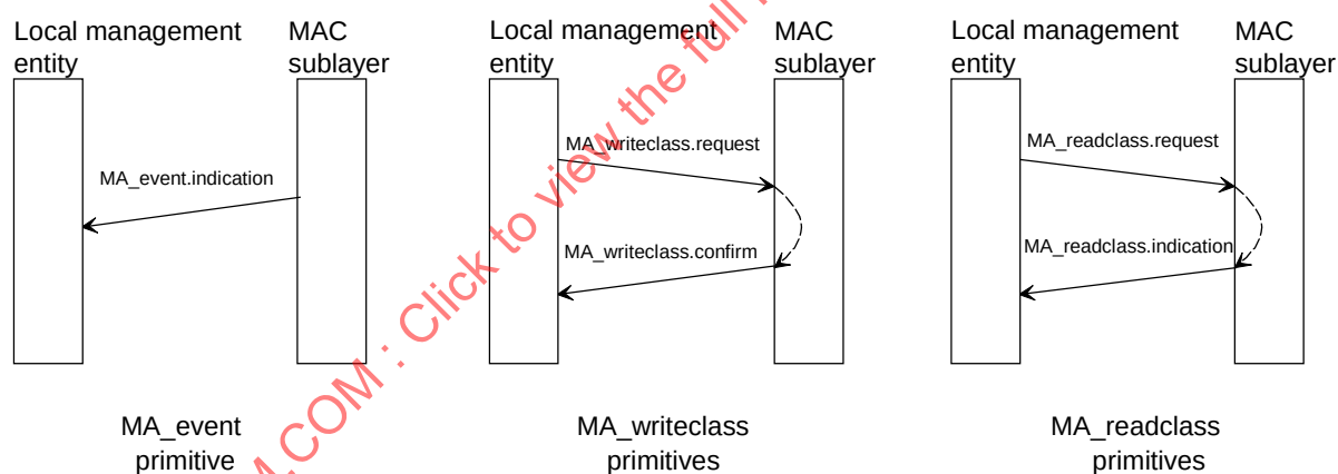
Figure 6 – MAC management services
