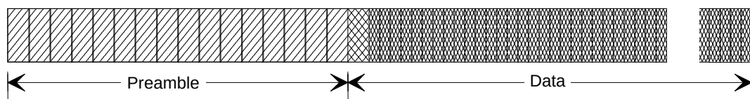
Figure 3 – Actual P_PDU representation
