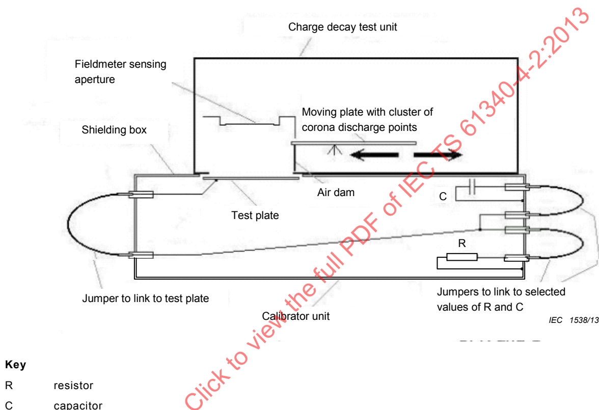
Figure D.2 – Equipment for charge decay time calibration
