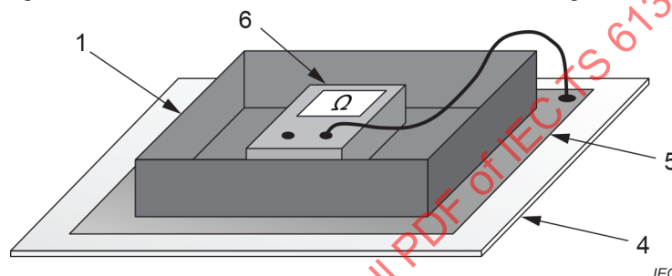
a) Test using resistance measurement electrode or concentric ring electrode assembly
