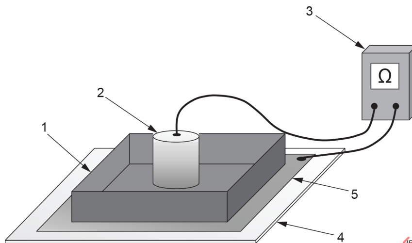
a) Test using resistance measurement electrode or concentric ring electrode assembly
