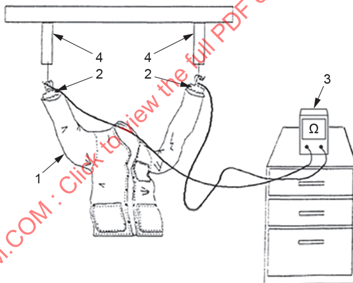
Figure 16 – Electrodes for hanging garment test
