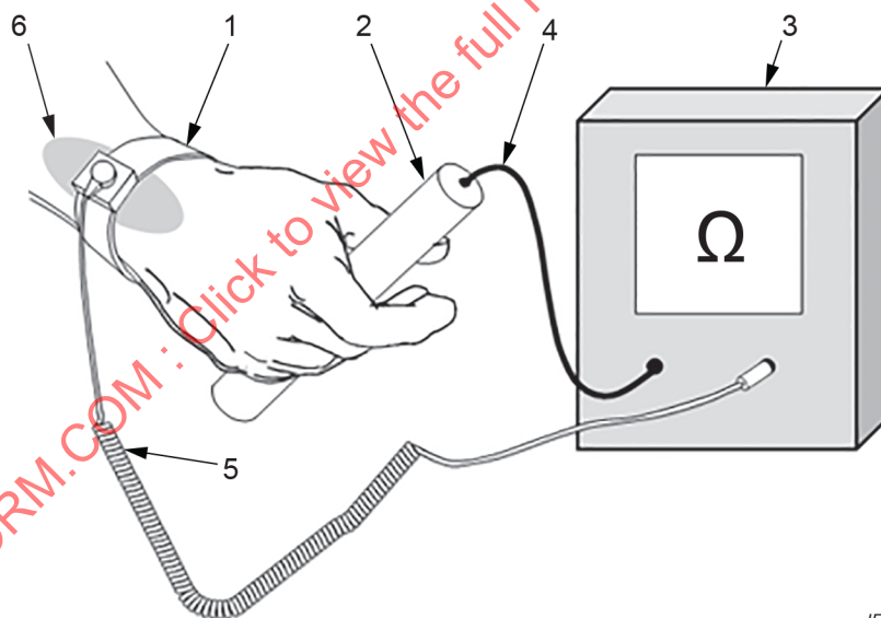
Figure 5 – Wrist strap test using resistance measurement apparatus
