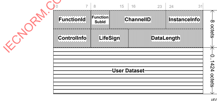
Figure 9 – Structure of function data unit
