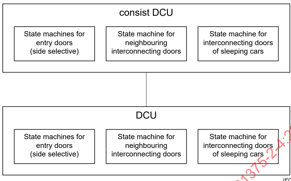
Figure 34 – State machine structure of DCU and consist DCU
