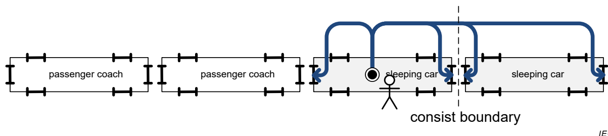
Figure 28 – Communication path for interconnecting doors of sleeping cars
