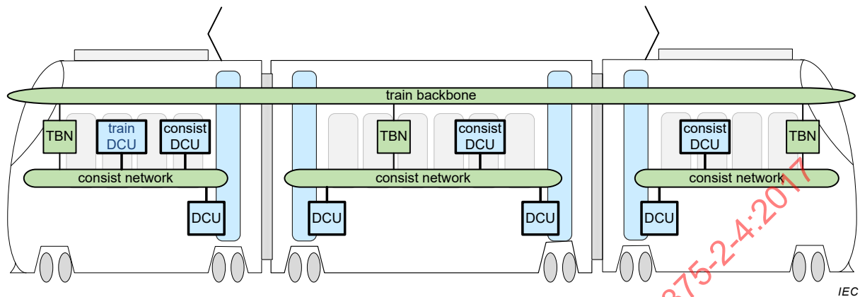
Figure 22 – Distribution structure of the door application
