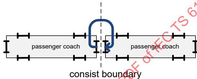
Figure 26 – Communication path for interconnecting doors
