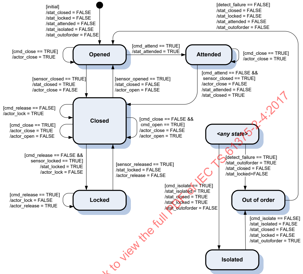
Figure 35 – DCU state diagram for entry doors
