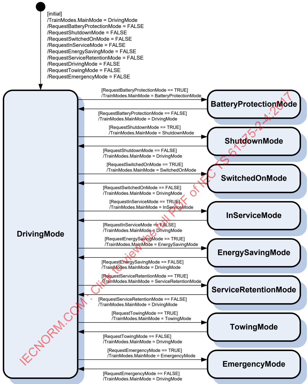
Figure 20 – Example train modes state diagram
