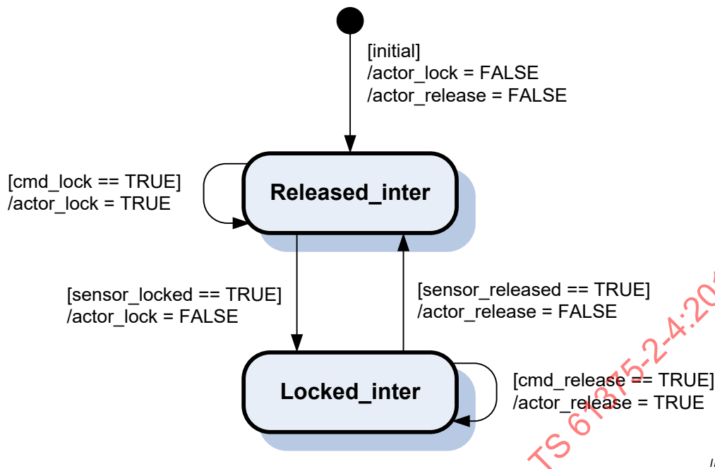
Figure 37 – DCU state diagram for interconnecting doors of sleeping cars
