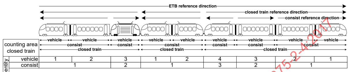
Figure 14 – Example sequence numbers in counting area closed train
