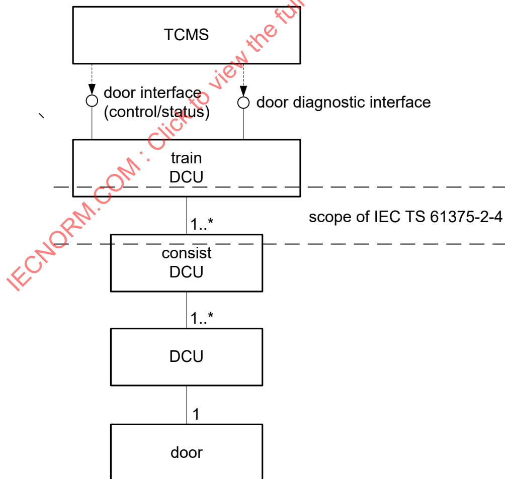
Figure 23 – Architecture of the door system
