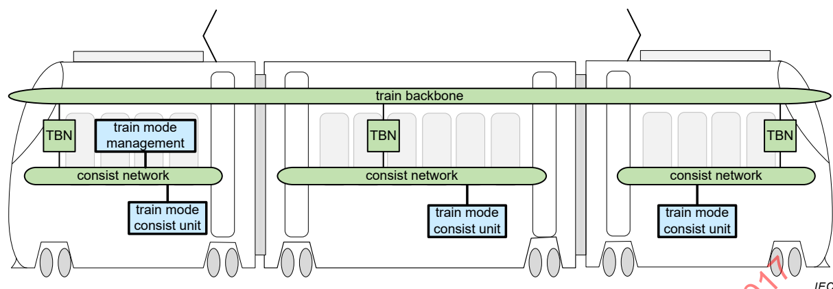
Figure 17 – Distribution structure for the function train mode
