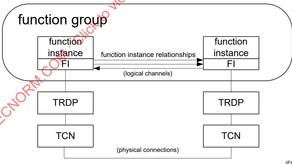
Figure 7 – Mapping of function instance relations to communication infrastructure
