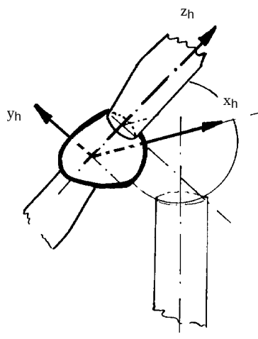
Figure A.2 – Hub co-ordinate system
