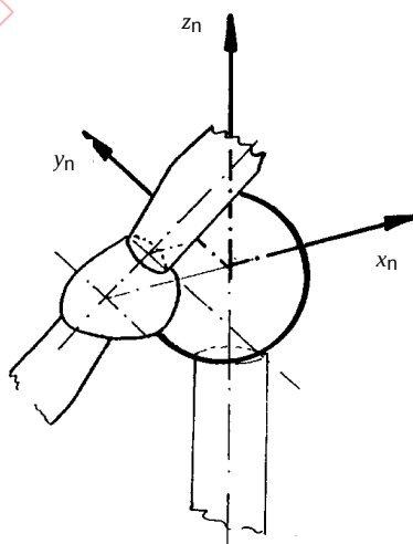
Figure A.3 – Nacelle co-ordinate system
