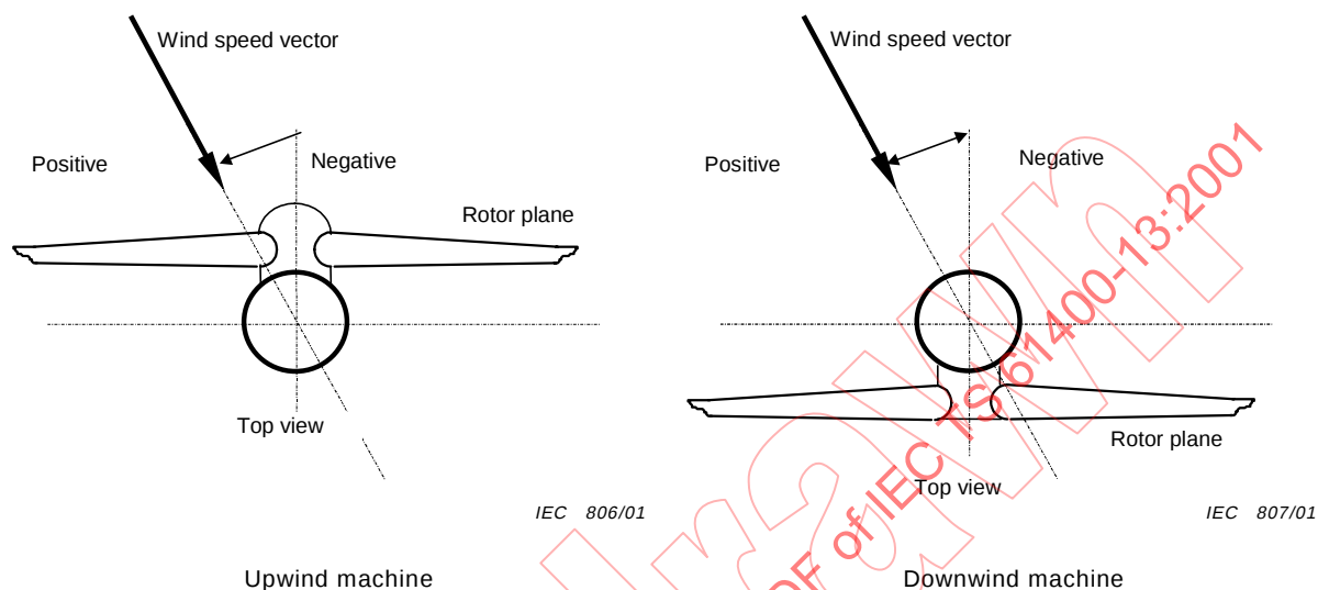
Figure A.5 – Yaw misalignment
