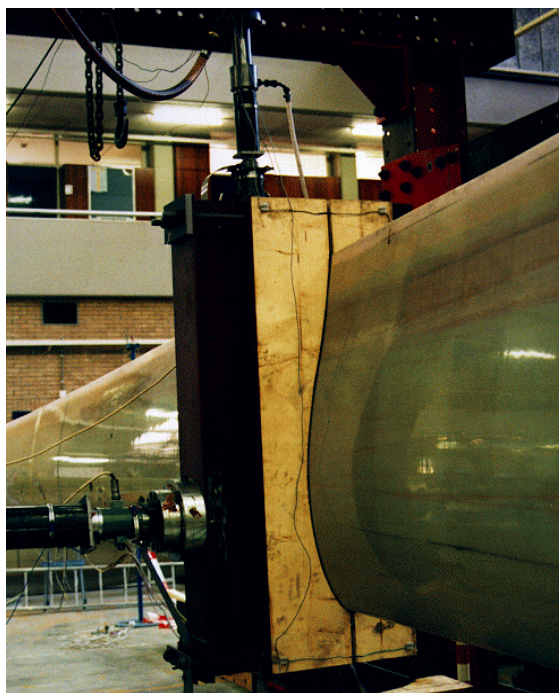
Figure 6 – Blade attachment fixture using an external sleeve of wood.
