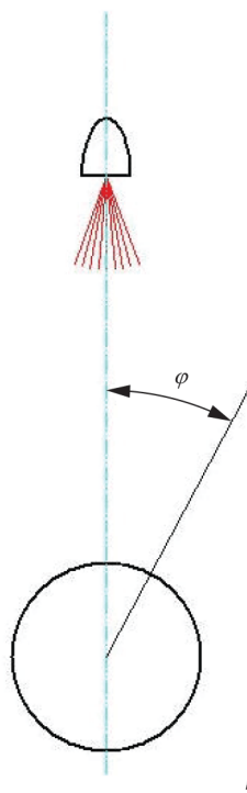
Figure CC.1 – Illumination model – Sphere illuminated by a point source
