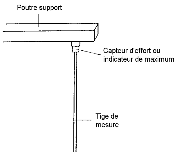
Figure C.2c – Type vertical
