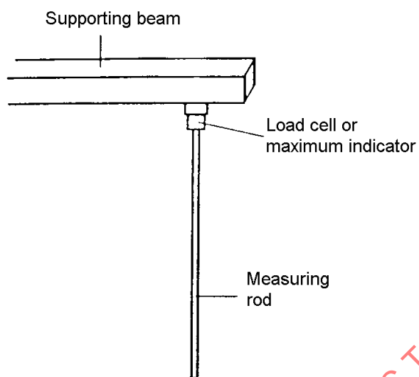
Figure C.2c – Vertical type
