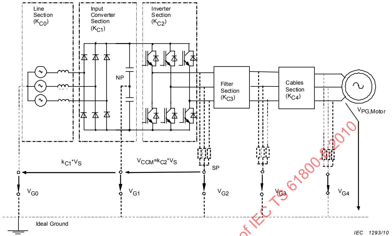
Figure 13 – Equivalent circuit diagram for calculation of the common mode voltage
