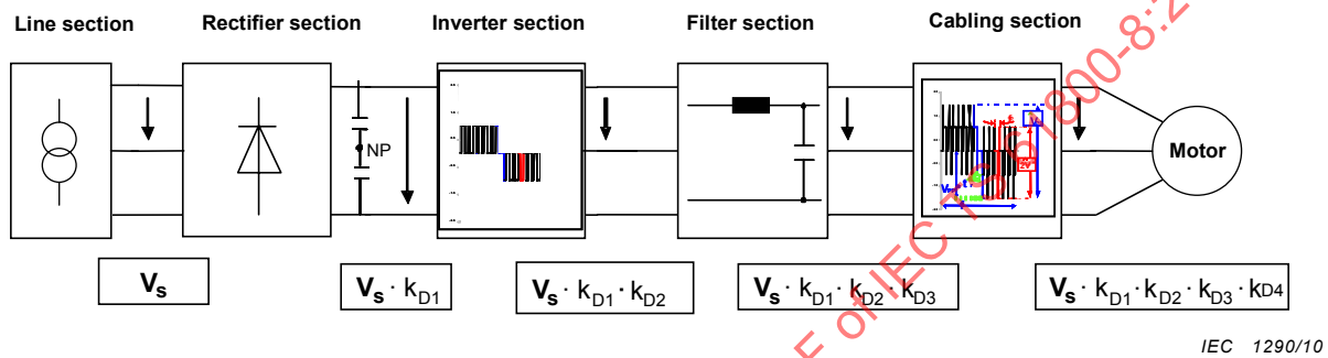
Figure 10 – Block diagram of two-port elements to achieve the motor terminal voltage in the differential mode model
