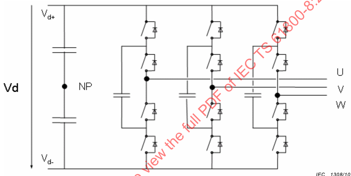
Figure 29 – Topology of a N = 3 level voltage source inverter (floating symmetrical capacitor)
