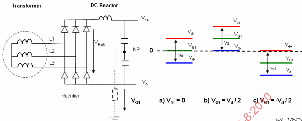
Figure 21 – Voltage source with three phase diode rectifier supplied by an IT supply system
