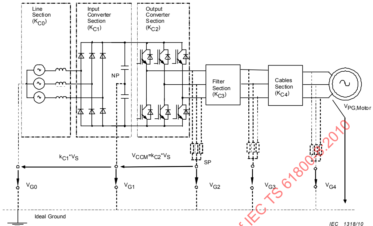
Figure 39 – Common Mode Equivalent Circuit
