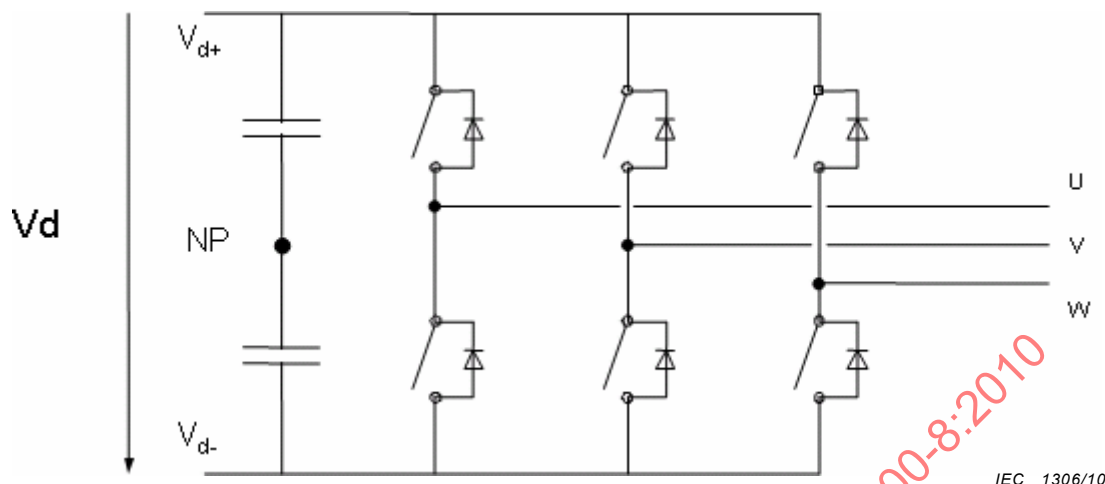
Figure 27 – Topology of a N = 2 level voltage source inverter
