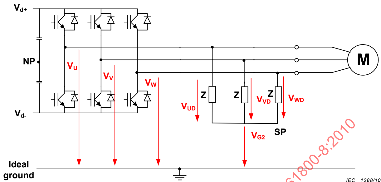
Figure 8 – Differential mode and common mode voltage system
