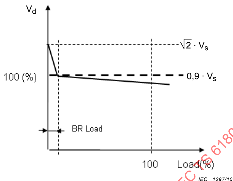
Figure 18 – Typical DC voltage V_d of single phase diode rectifier without braking mode. BR is the bleeder resistor to discharge the capacitor
