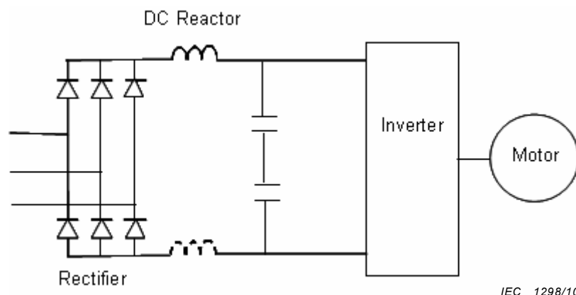
Figure 19 – Typical configuration of a voltage source inverter with three phase diode rectifier
