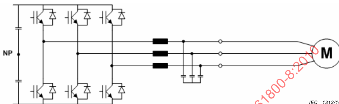
Figure 33 – Topology of a differential mode sine wave filter
