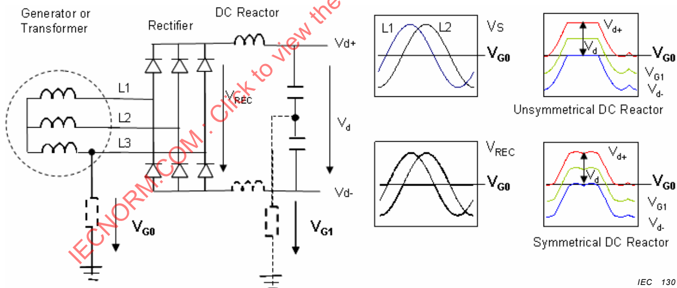
Figure 22 – Voltage source with three phase diode rectifier supplied from a delta grounded supply system
