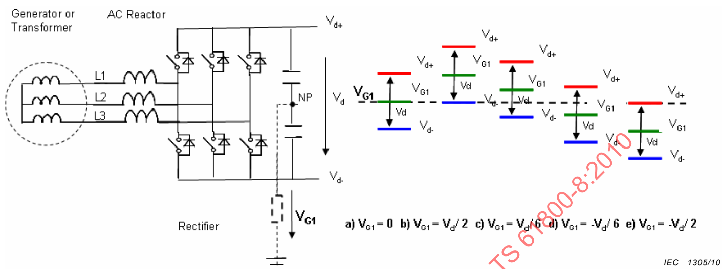
Figure 26 – Voltage source with three phase active infeed supplied by a IT supply system
