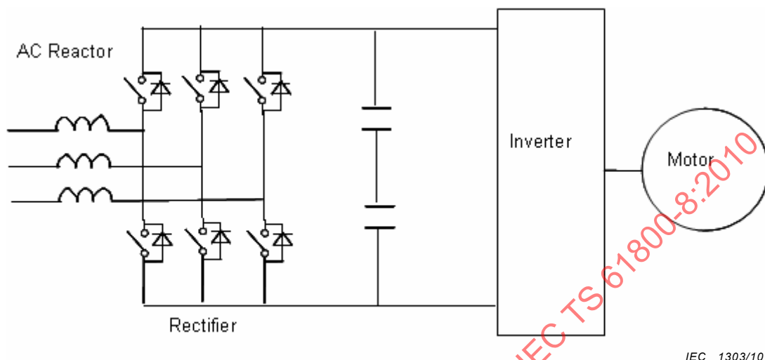
Figure 24 – Typical configuration of a VSI with three phase active infeed converter
