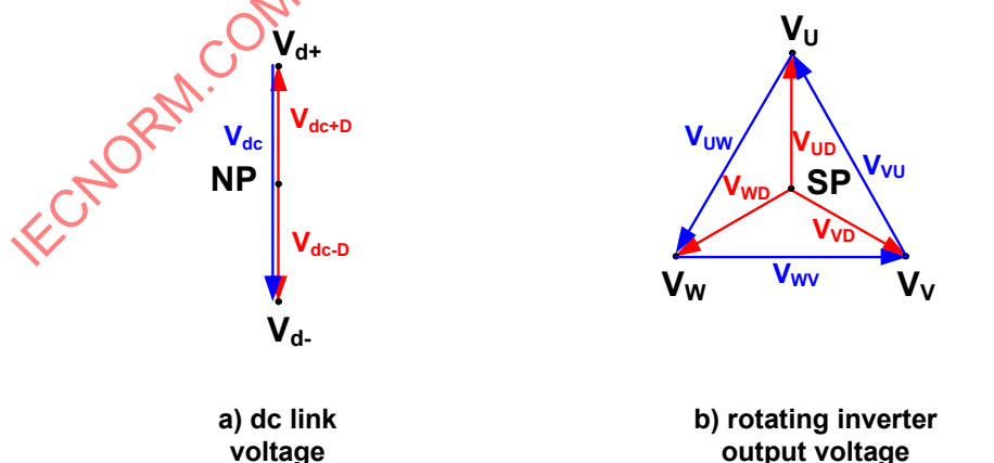
Figure 9 – Voltages in the differential mode system
