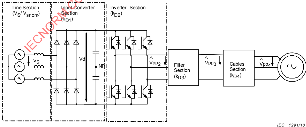
Figure 11 – Equivalent circuit diagram for calculation of the differential mode voltage
