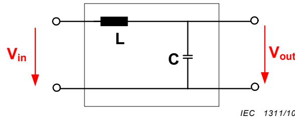
Figure 32 – Basic filter topology
