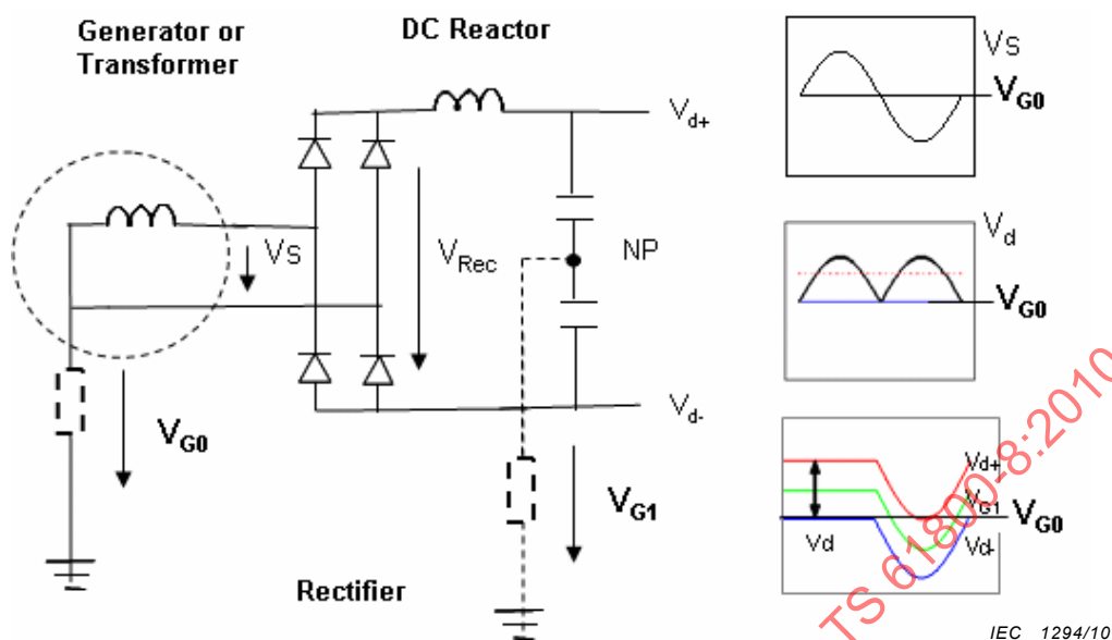
Figure 15 – Typical configuration of a voltage source inverter with single phase diode rectifier supplied by L and N from a TN or TT supply system
