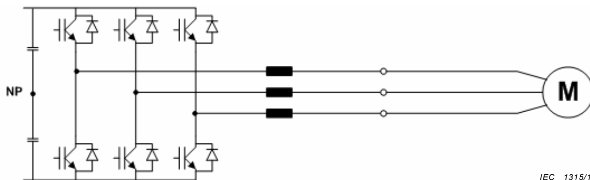
Figure 36 – Topology of the output choke
