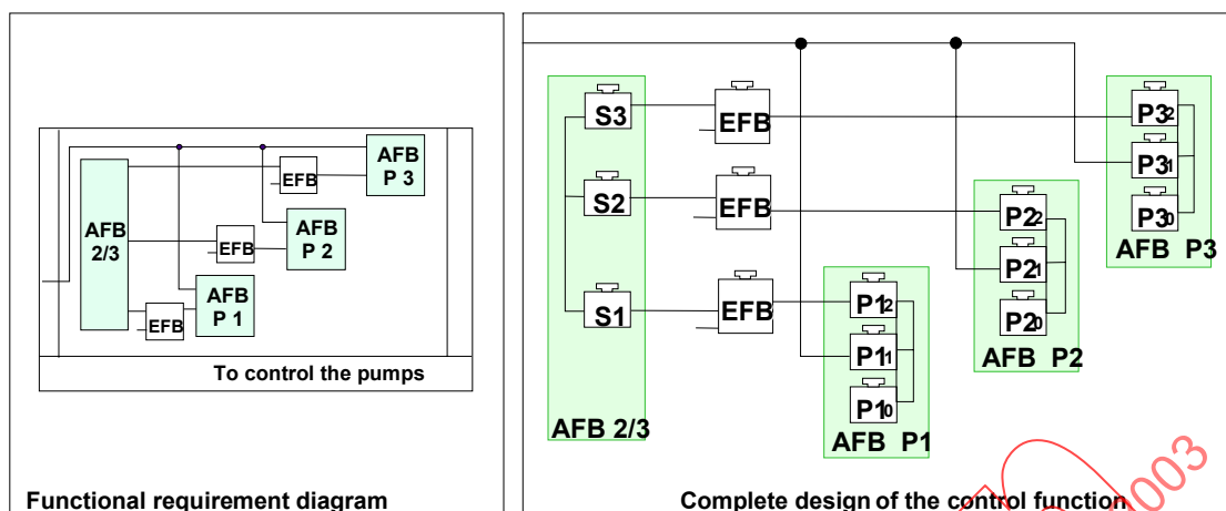
Figure A.23 – From a FRD to a programming scheme using IEC 61499-1 system model
