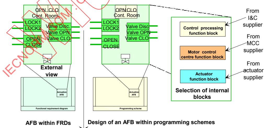
Figure A.16 – Designing internal behaviour of actuation AB from actuation device off the shelf
