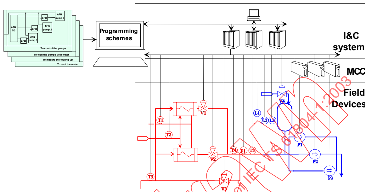
Figure A.14 – From FRDs down to the I&C system and devices
