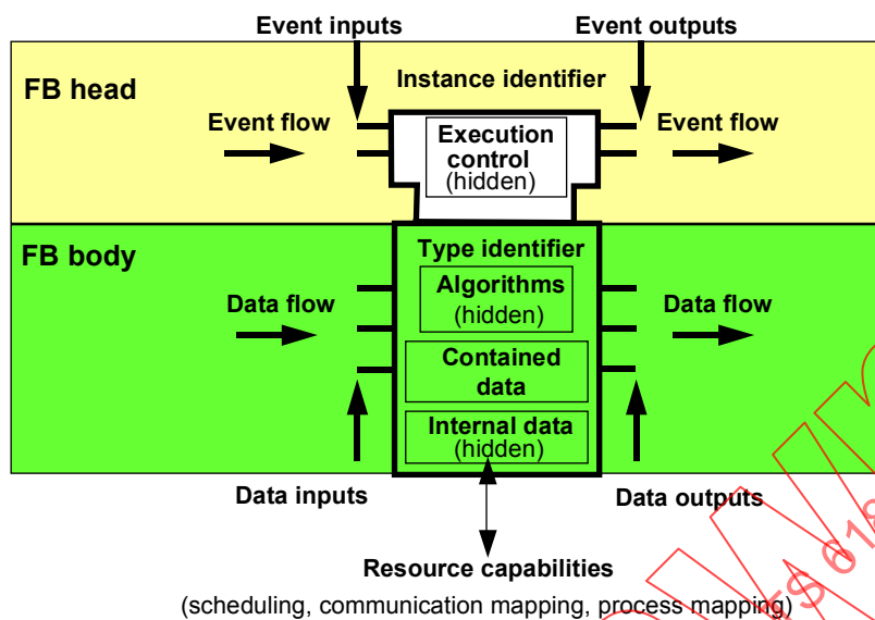
Figure C.1 – Structure of IEC 61499-1 FBs
