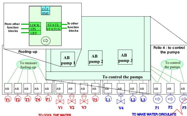
Figure A.8 – Selection of a folio from the CHD
