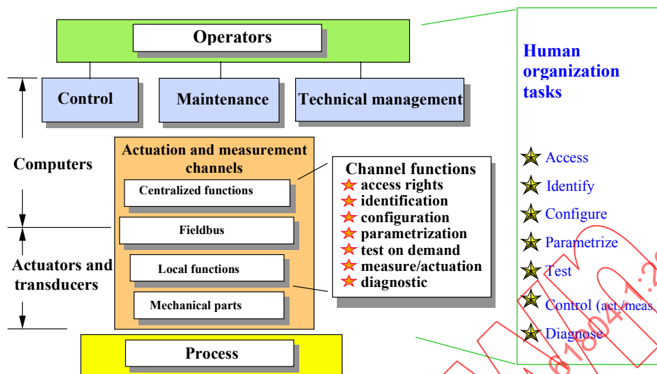
Figure B.3 – Reference functional architecture for distributed automation systems
