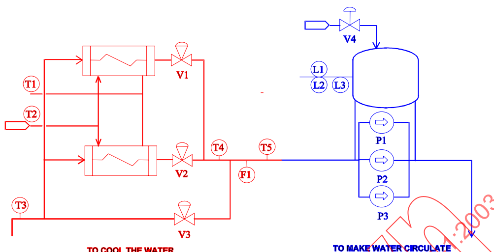
Figure A.2 – PFD composed of two process elementary operations
