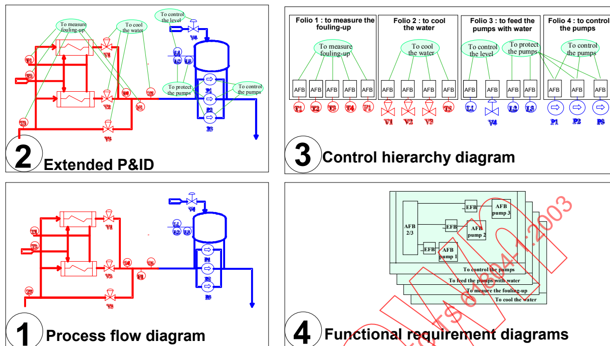
Figure A.1 – Life cycle from the process circuit to the FRDs
