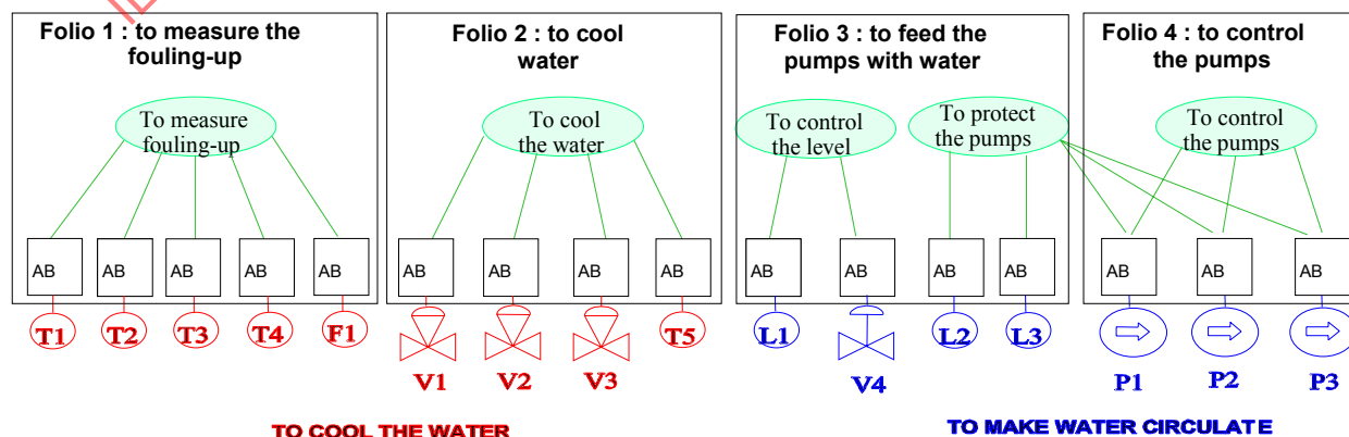
Figure A.6 – Structured documentation for the requirements of the control functions
