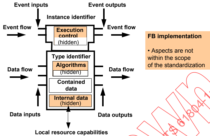
Figure C.3 – Implementation specific aspects
