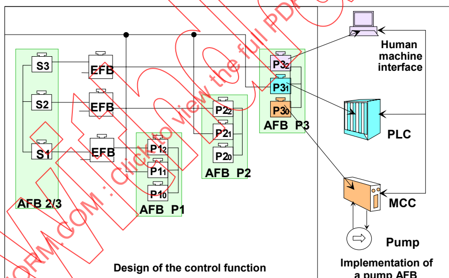
Figure A.24 – Distribution of the internal blocks of a pump AB
