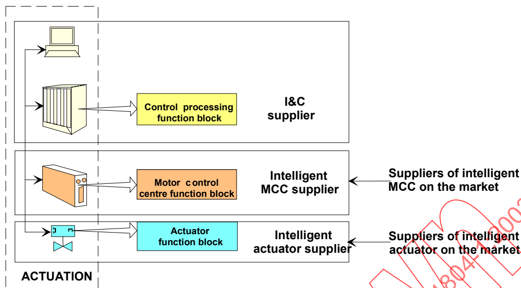
Figure A.15 – Design of an actuation and its AB from off-the-shelf actuation devices
