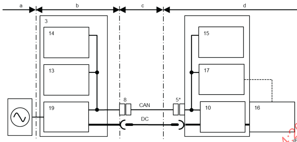
Figure 8 – Conversion device for configuration type C
