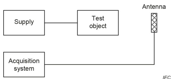
Figure 6 – Circuit using an electromagnetic UHF antenna
