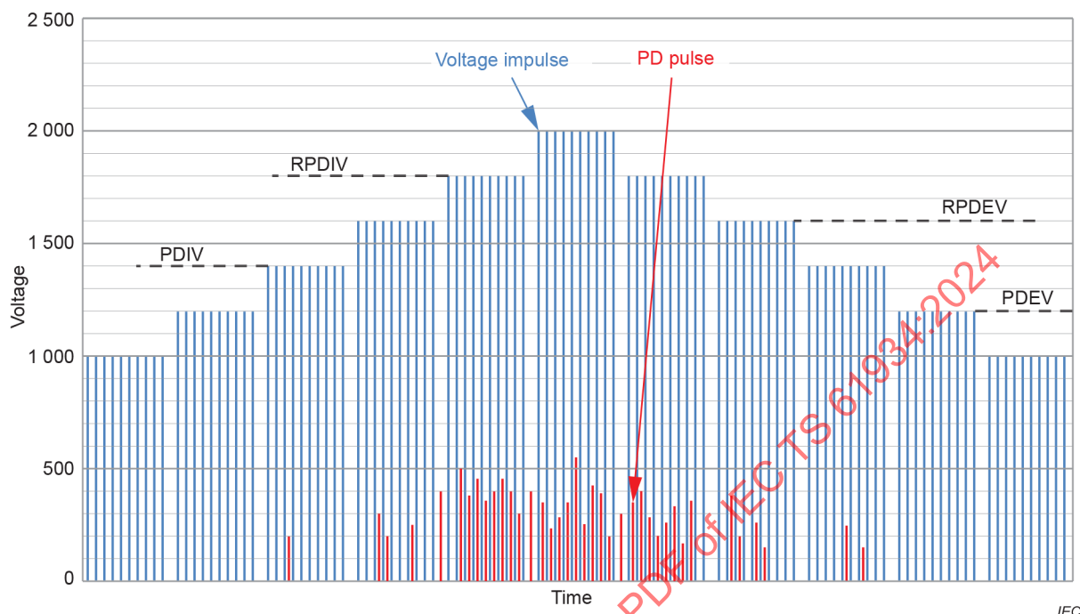
Figure 9 – Example of increasing and decreasing the impulse voltage magnitude
