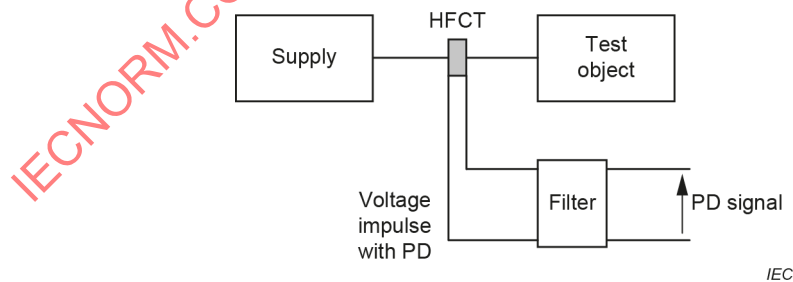
Figure 3 – HFCT between supply and test object with multipole filter
