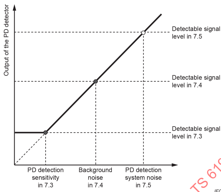
Figure 8 – Example of relation between the outputs of LVPG and PD detector
