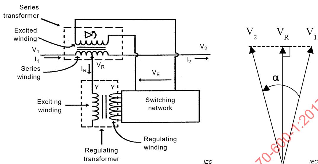
Figure D.12 – Symmetrical phase shifters with two cores
