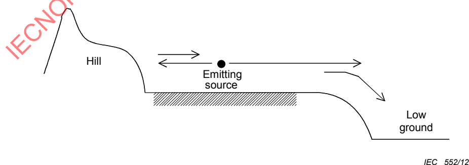
Figure 5 – Example of reflecting hill and low ground
