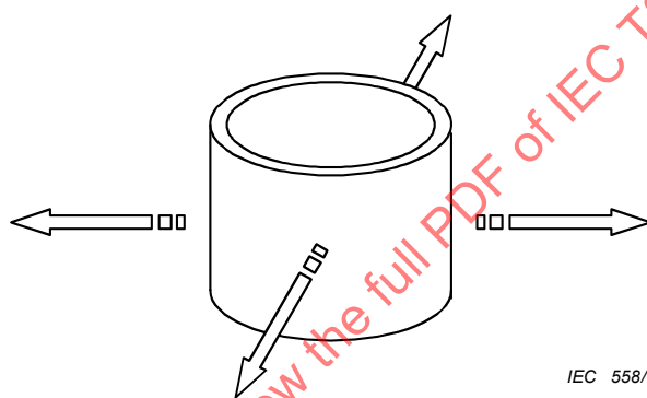
Figure 11 – Simplified shape of the symmetrical breathing mode of a reactor winding
