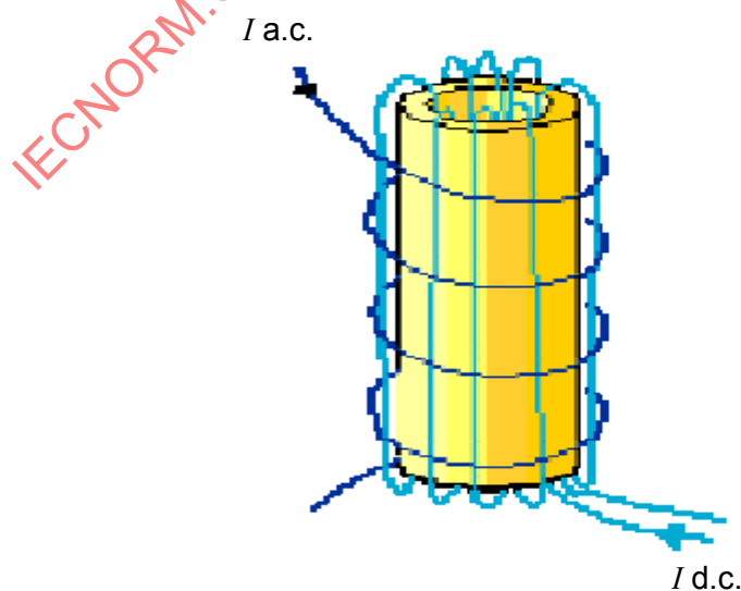
Figure 17 – Reactor for self-tuned filter applications
