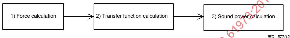
Figure 30 – Three steps to determine the sound power of HVDC components
