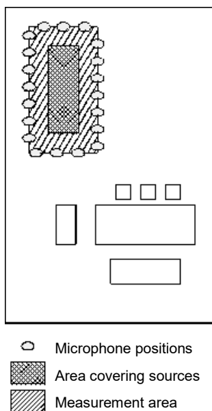
Figure 35 – HVDC substation and example of microphone positions for determination of sound power levels
