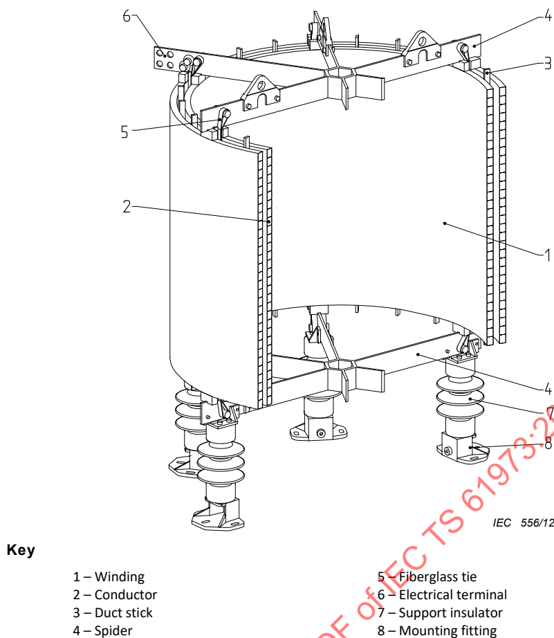
Figure 9 – Dry-type air-core reactor
