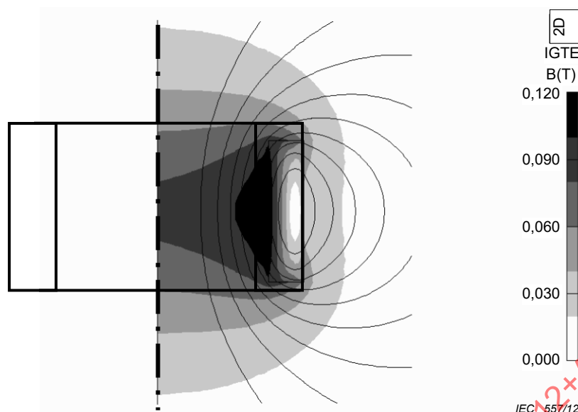
Figure 10 – Magnetic field of an air-core reactor winding
