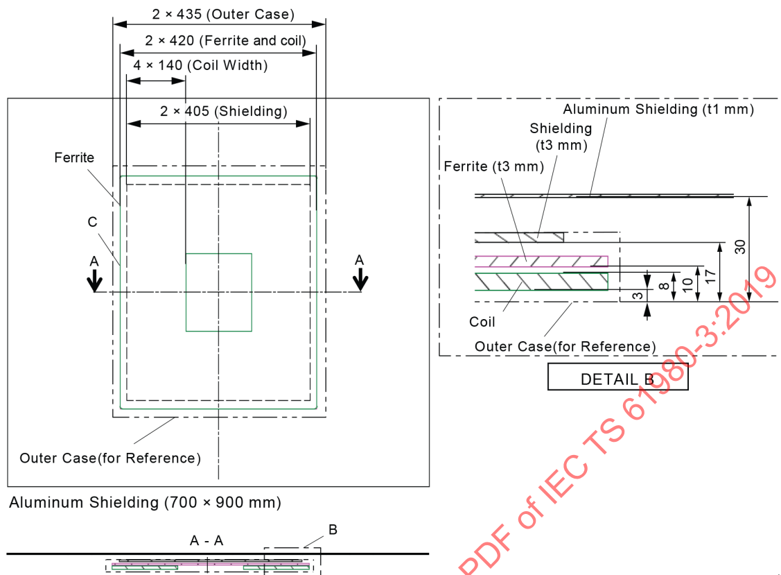
Figure BB.5 – Mechanical dimensions of the MF-WPT1/Z3 circular reference secondary device
