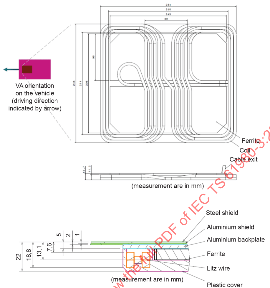
Figure AA.11 – Mechanical dimensions of the MF-WPT3/Z1 DD reference secondary device
