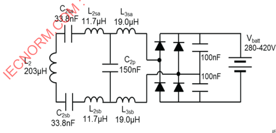
Figure BB.6 – Schematic of the EV power electronics for the MF-WPT1/Z3 circular reference EVPC
