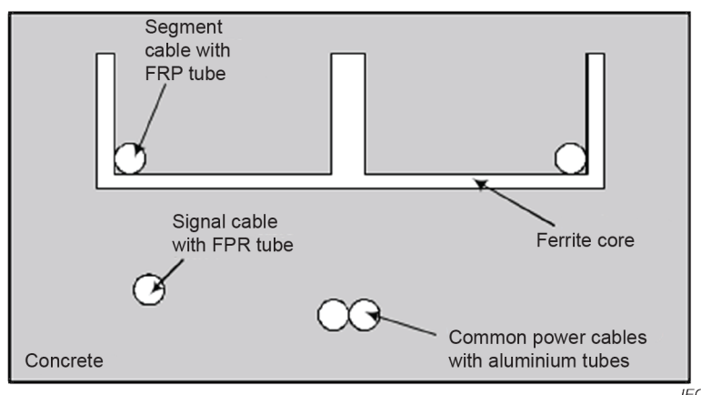
Figure CC.1 – Mechanical dimensions of the MF-WPT5 heavy-duty WPT reference primary device
