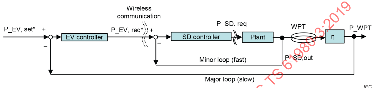
Figure 104 – Control loop of WPT system
