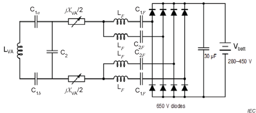
Figure BB.18– Schematic of the EV power electronics for the MF-WPT3/Z3 circular reference EVPC
