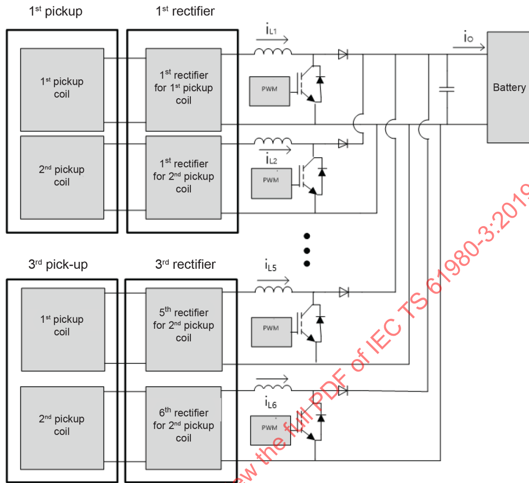
Figure CC.4 – Schematic of the EV power electronics for the MF-WPT5 heavy-duty WPT secondary reference device
