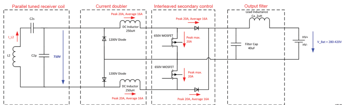
Figure AA.12 – Schematic of the EV power electronics for the MF-WPT3/Z1 DD reference EVPC
