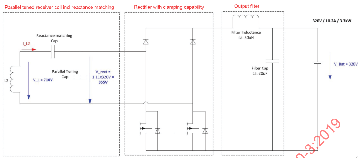
Figure AA.2 – Schematic of the EV power electronics for the MF-WPT1/Z1 DD reference EVPC
