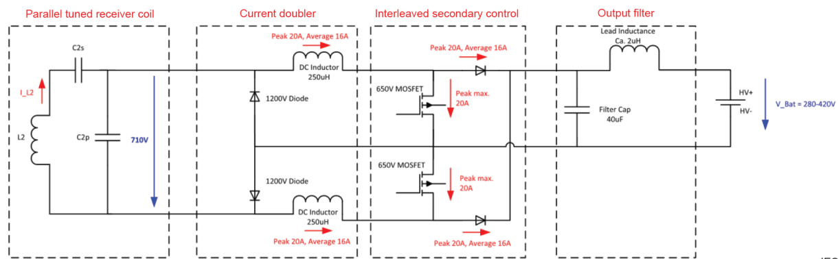
Figure AA.14 – Schematic of the EV power electronics for the MF-WPT3/Z2 DD reference EVPC
