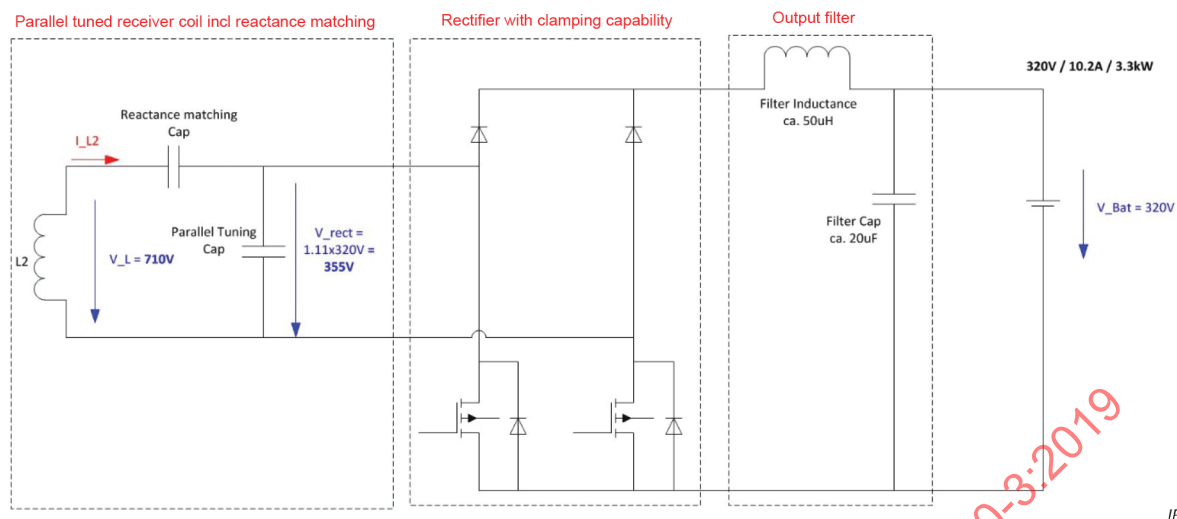
Figure AA.4 – Schematic of the EV power electronics for the MF-WPT1/Z2 DD reference EVPC
