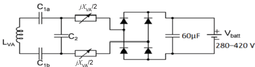
Figure BB.8 – Schematic of the EV power electronics for the MF-WPT2/Z1 circular reference EVPC
