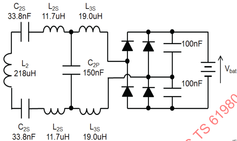
Figure BB.4– Schematic of the EV power electronics for the MF-WPT1/Z2 circular reference EVPC
