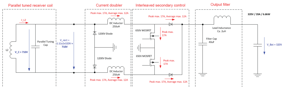
Figure AA.8 – Schematic of the EV power electronics for the MF-WPT2/Z2 DD reference EVPC
