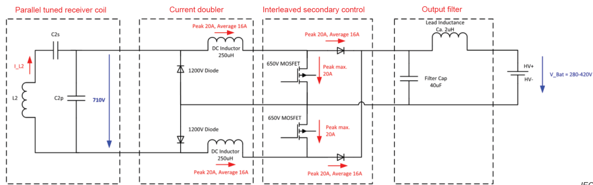
Figure AA.16 – Schematic of the EV power electronics for the MF-WPT3/Z3 DD reference EVPC
