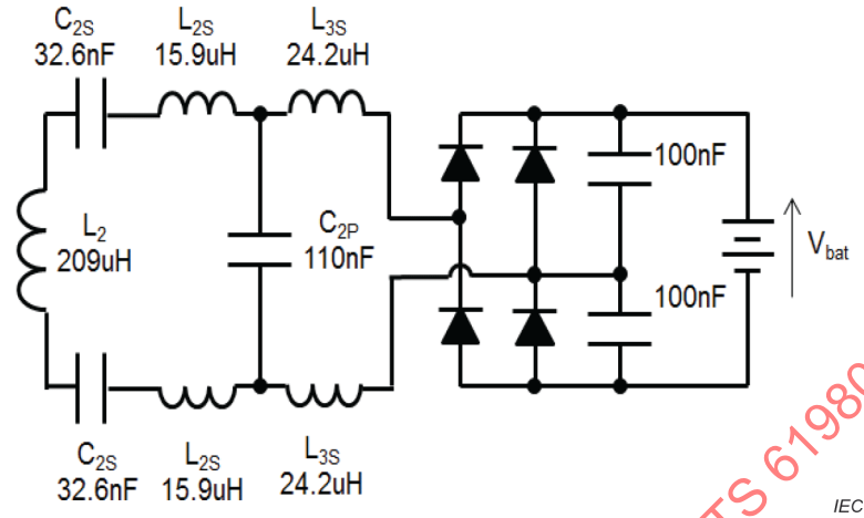
Figure BB.2 – Schematic of the EV power electronics for the MF-WPT1/Z1 circular reference EVPC
