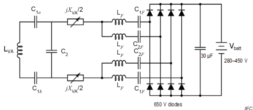
Figure BB.16 – Schematic of the EV power electronics for the MF-WPT2/Z2 circular reference EVPC
