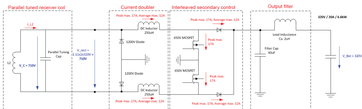
Figure AA.10 – Schematic of the EV power electronics for the MF-WPT2/Z3 DD reference EVPC
