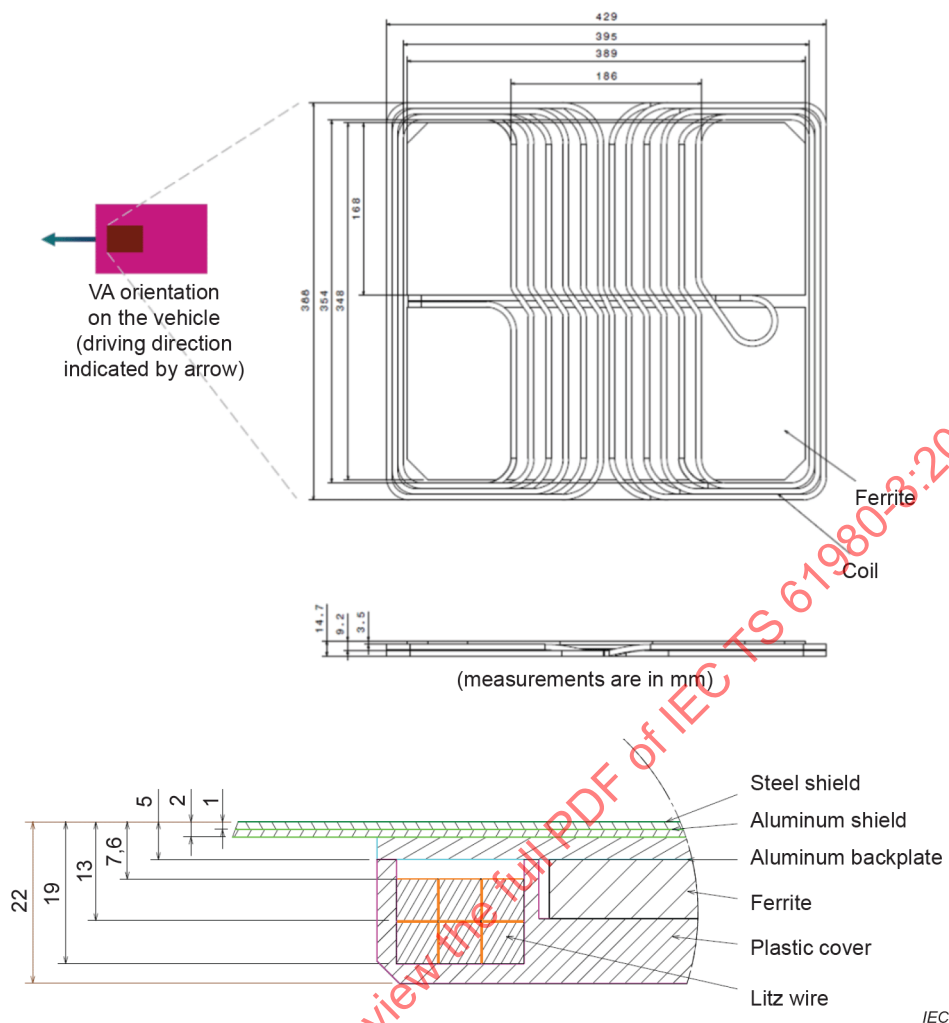
Figure AA.15 – Mechanical dimensions of the MF-WPT3/Z3 DD reference secondary device
