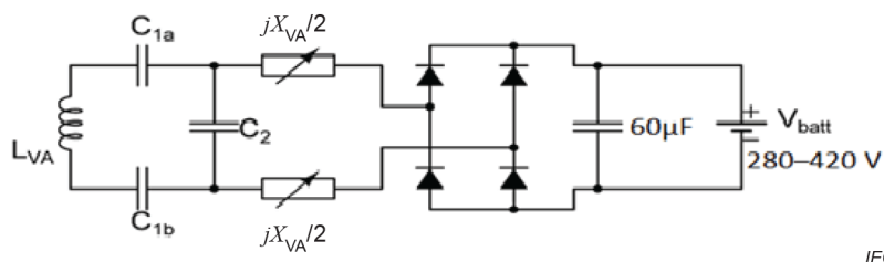
Figure BB.12 – Schematic of the EV power electronics for the MF-WPT2/Z3 circular reference EVPC
