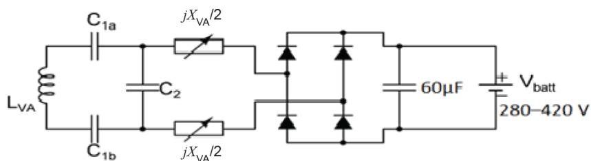
Figure BB.10 – Schematic of the EV power electronics for the MF-WPT2/Z2 circular reference EVPC
