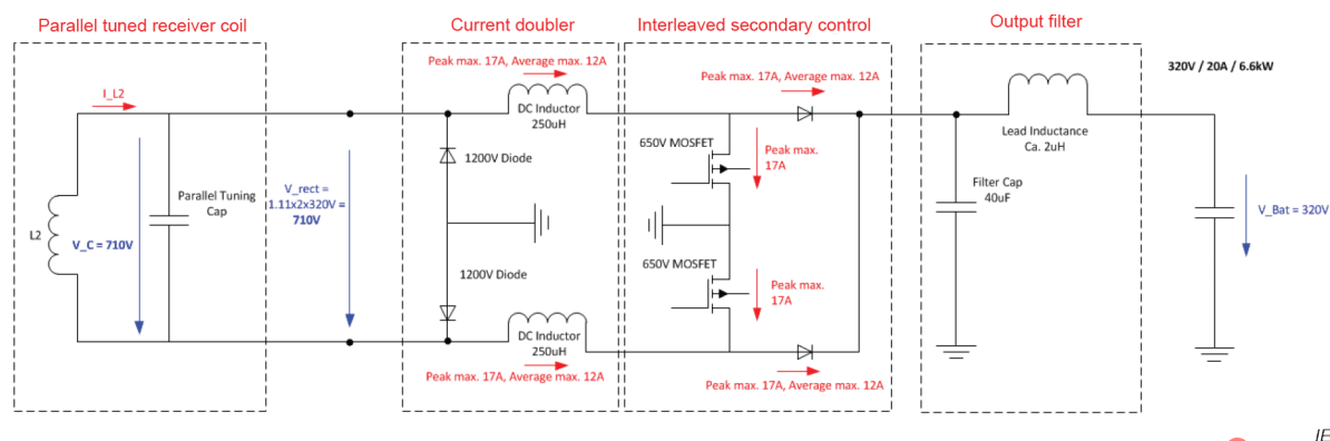
Figure AA.6 – Schematic of the EV power electronics for the MF-WPT2/Z1 DD reference EVPC
