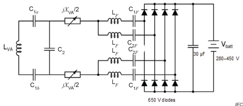
Figure BB.14 – Schematic of the EV power electronics for the MF-WPT3/Z1 circular reference EVPC
