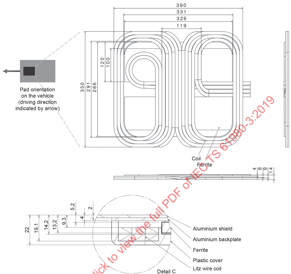
Figure AA.9 – Mechanical dimensions of the MF-WPT2/Z3 DD reference secondary device
