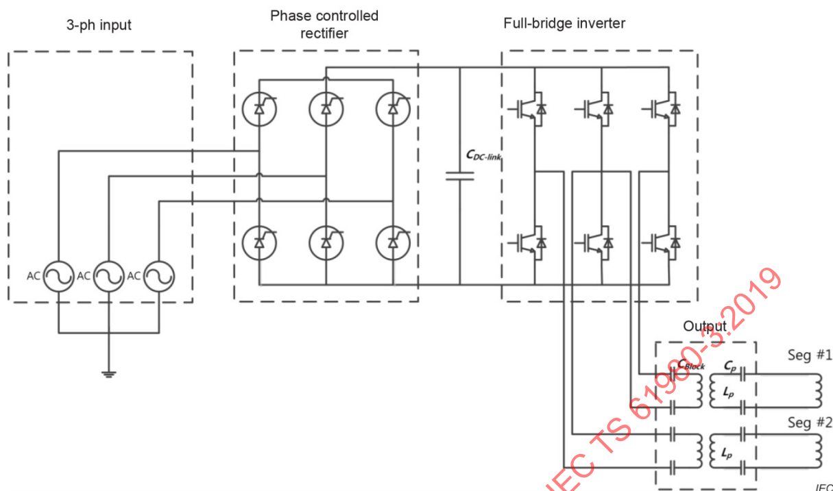
Figure CC.2 – Schematic of supply power electronics for the heavy-duty WPT reference primary device
