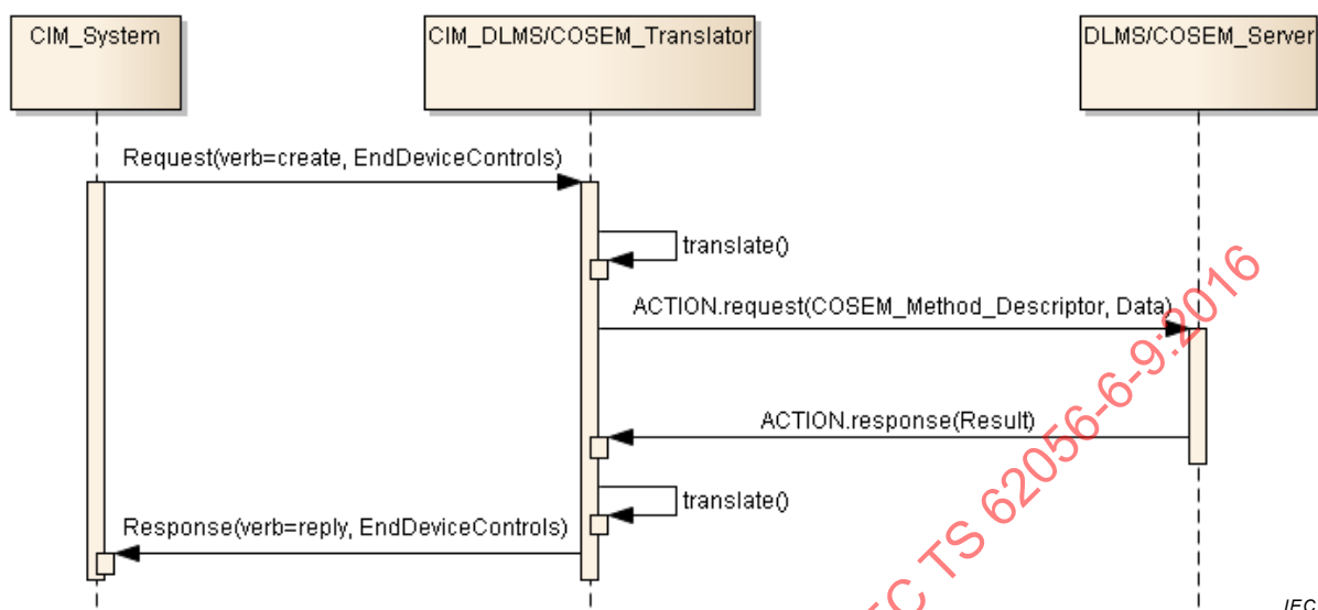
Figure 7 – UC5: ManageLoadByRelayControl
