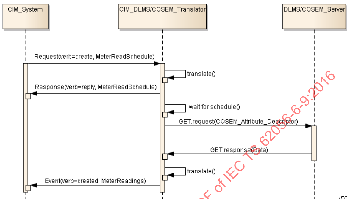
Figure 8 – UC6: ReportOnQualityOfSupply
