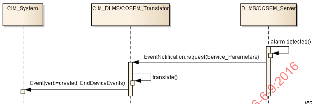
Figure 13 – UC11: SuperviseMeter
