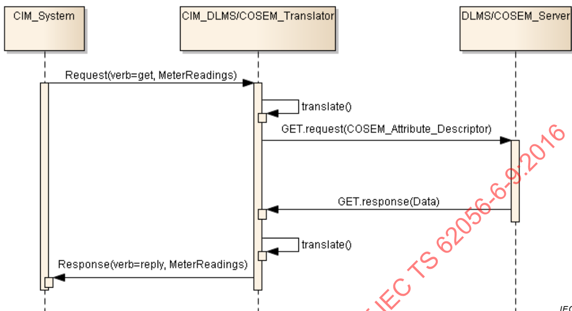
Figure 4 – UC2: ReadMeterOnDemand
