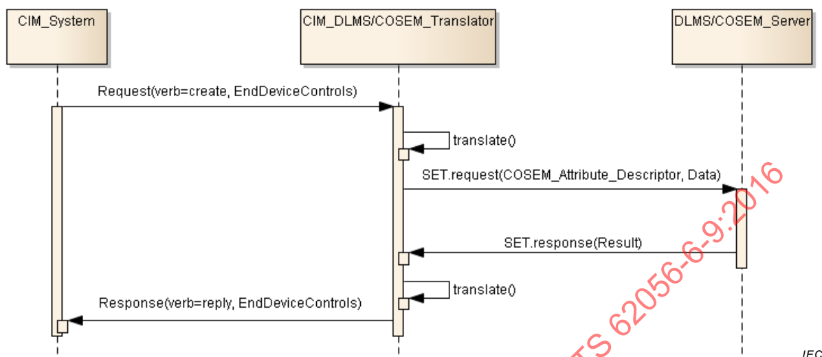
Figure 9 – UC7: ManageLoadByDemandLimits
