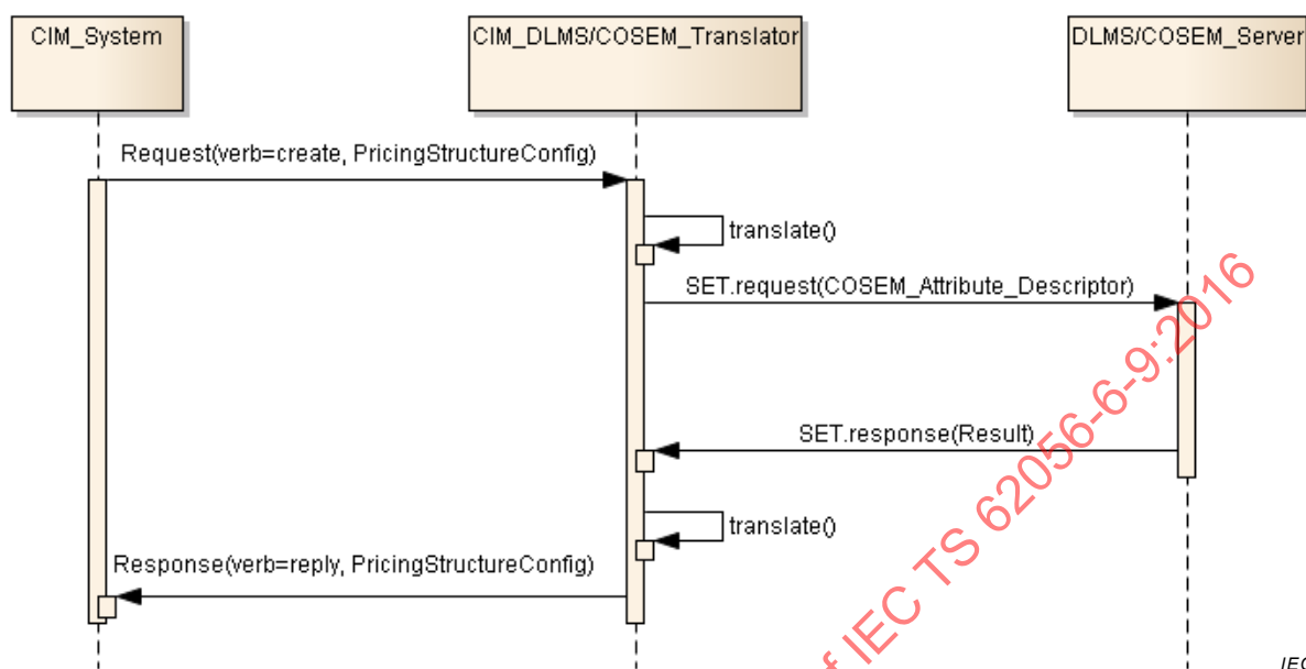
Figure 5 – UC3: ConfigureTariffRemotely
