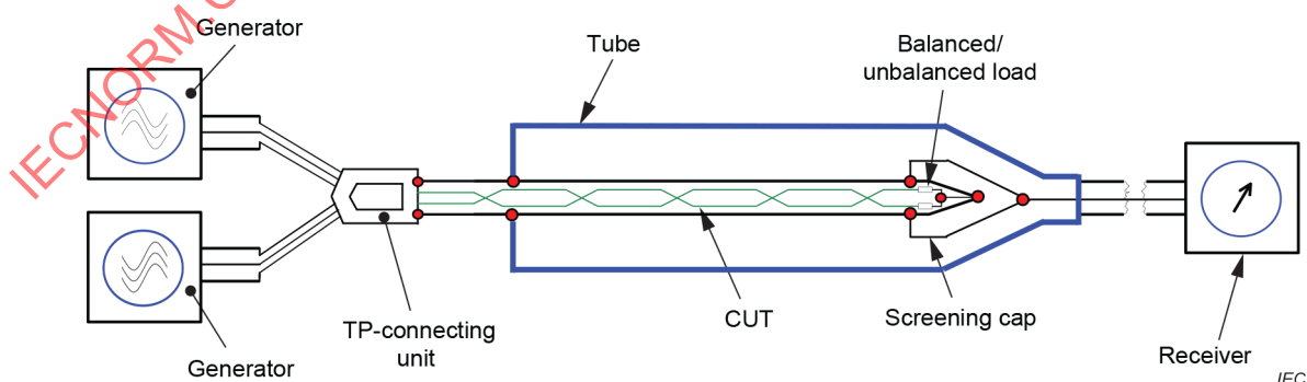
Figure A.5 – Balunless measuring of coupling attenuation, principle set-up with multiport VNA and standard head
