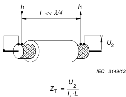
Figure 43 – Definition of transfer impedance
