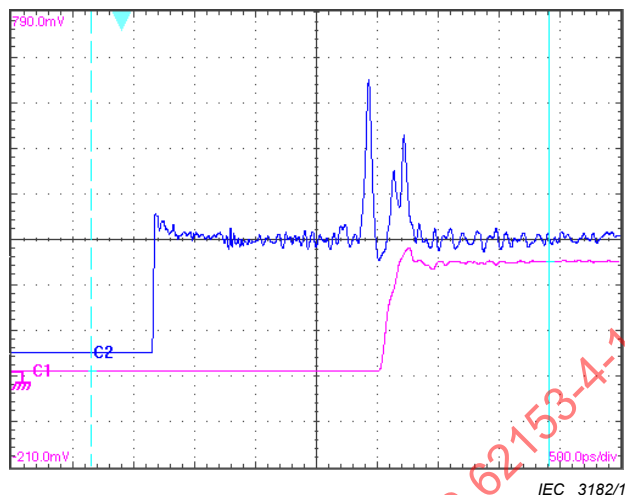
Figure 68 – TDR step response from A (Input)-port of test fixture with inserted “Teflon-through” sample
