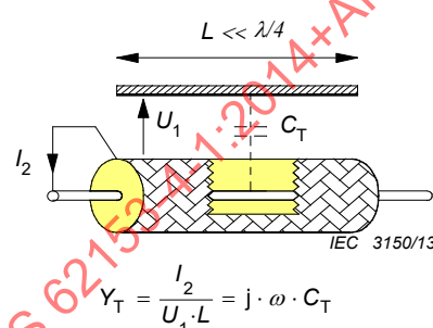
Figure 44 – Definition of coupling admittance
