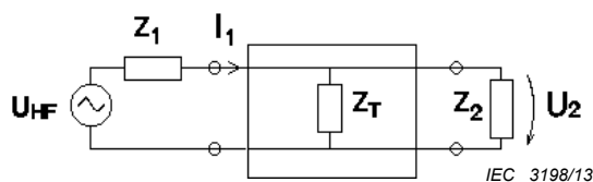
Figure 82 – equivalent circuit of the set-up with inserted DUT
