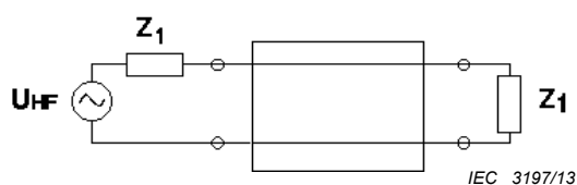
Figure 81 – equivalent circuit of the set-up without DUT
