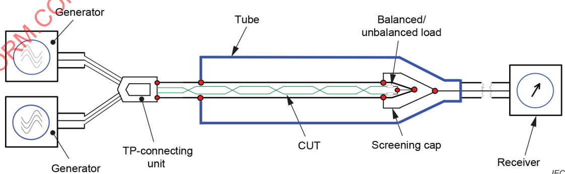
Figure A.5 – Balunless measuring of coupling attenuation, principle set-up with multiport VNA and standard head
