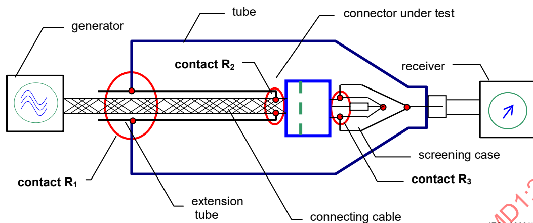
Figure 91 – Contact resistances of the test set-up
