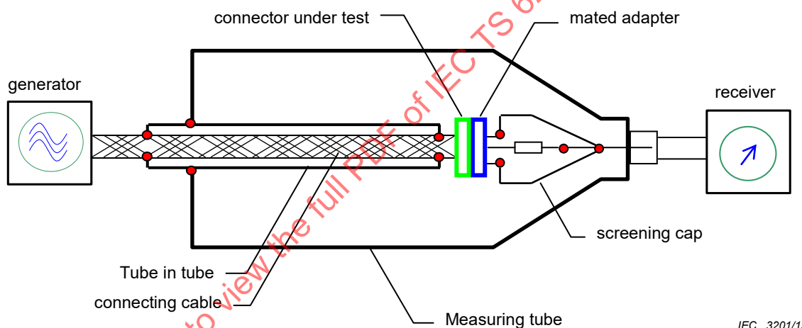
Figure 85 – Principle test set-up for measuring the screening attenuation of a connector with the tube in tube procedure
