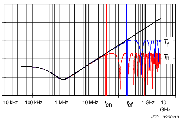
Figure 84 – Calculated coupling transfer function
