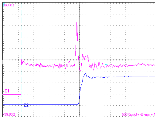
Figure 67 – TDR measurement of the text-fixture with inserted “Teflon-through” sample
