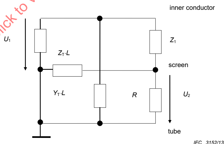
Figure 46 – Equivalent circuit of the triaxial measuring set-up
