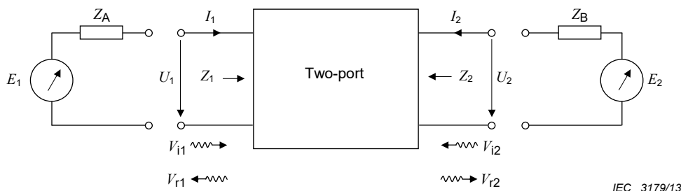
Figure 66 – Two-port network
