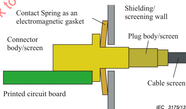
Figure 63 – Cross-sectional sketch of a typical feed-through configuration
