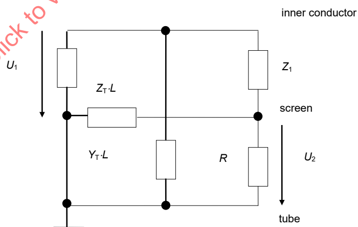
Figure 45 – Triaxial measuring set-up for screening attenuation
