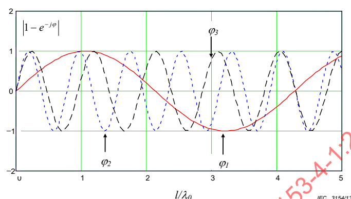
Figure 48 – Calculated periodic functions for \epsilon_{r1} = 2,3 and \epsilon_{r2} = 1,1
