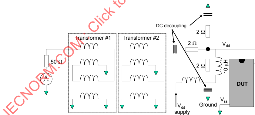
Figure 6 – Method to impose synchronous transient injection into supply/ V_{dd} pin(s)
