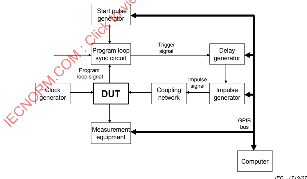
Figure 8 – Measurement set-up for synchronous transient injection
