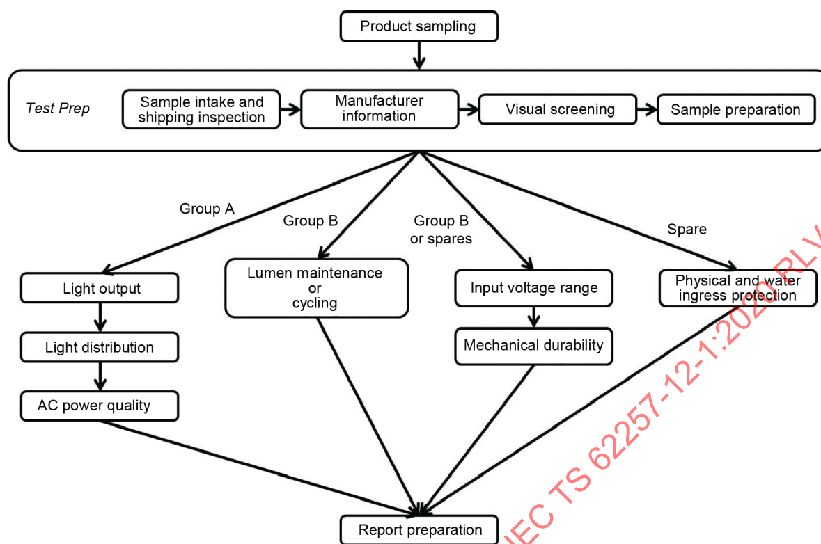
Figure 1 – Recommended sequence of testing for QTM
