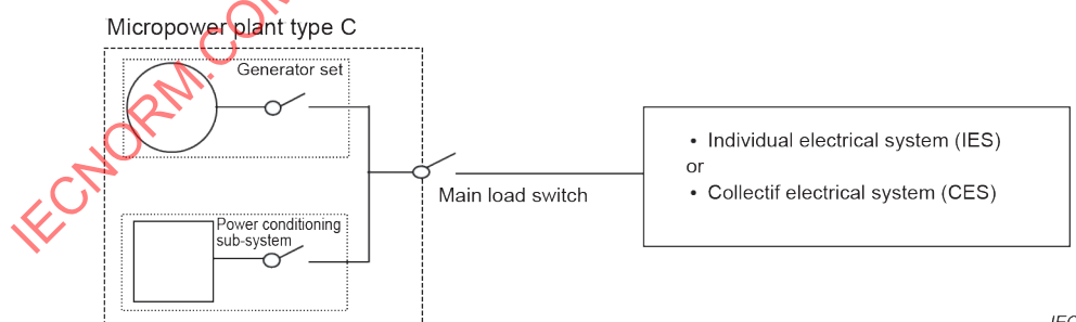
Figure 4 – Micropower plant Type C: single generator set with a power conditioning sub-system in micropower plant
