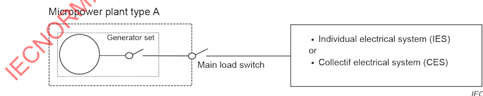
Figure 2 – Micropower plant Type A: single generator set
