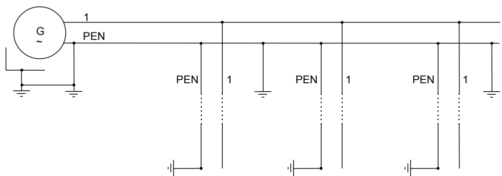
Figure 2 – Microgrid consisting of a single-phase feeder
