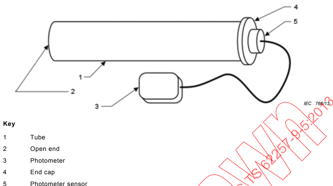
Figure J.1 – Schematic of a photometer tube
