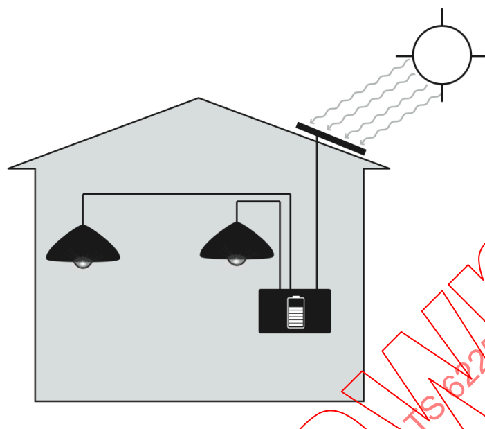
Figure 1 – Fixed indoor components – Example
