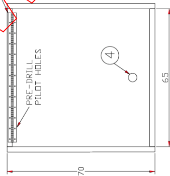
Figure Y.3 – Photometer box dimensions
