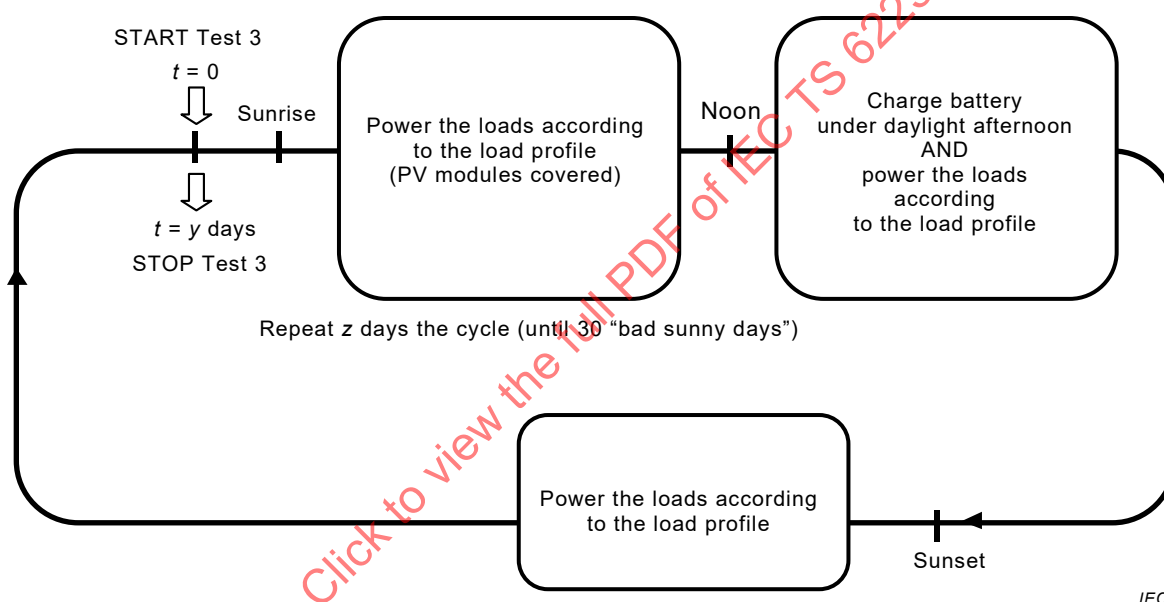
Figure 3 – Test 3, operating cycles
