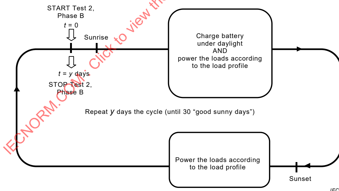
Figure 2 – Test 2, Phase B: operating cycles
