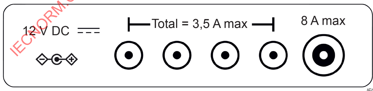
Figure 3 – Example labelling for a product with four ports having a combined current limit of 3,5 A and a separate port having a current limit of 8 A. The five ports together can supply a total of 11,5 A
