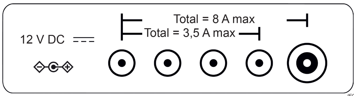
Figure 4 – Example labelling for a product with five ports having a combined current limit of 8 A and a subset of four ports having a combined current limit of 3,5 A
