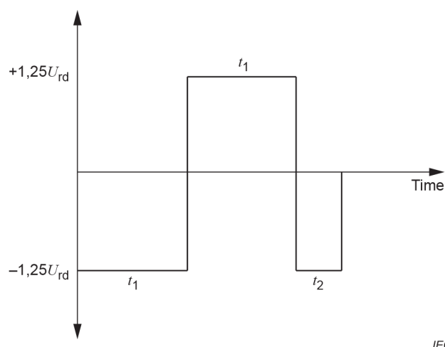
Figure 5 – Test sequence for polarity reversal tests
