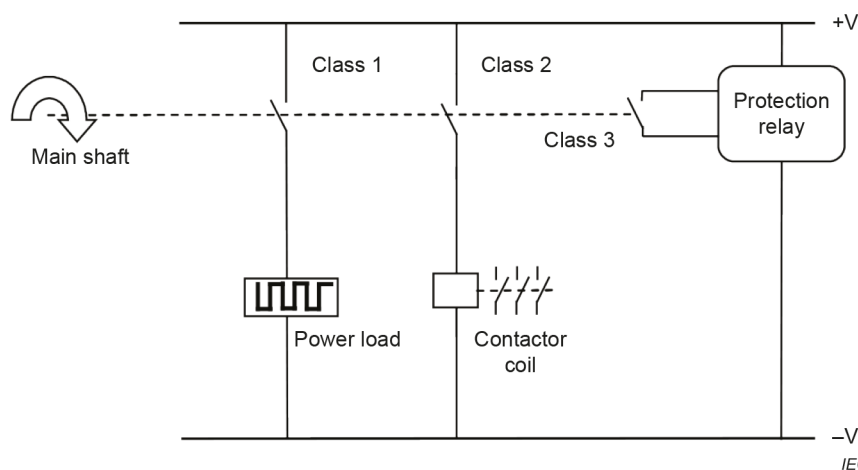
Figure 3 – Examples of classes of contacts
