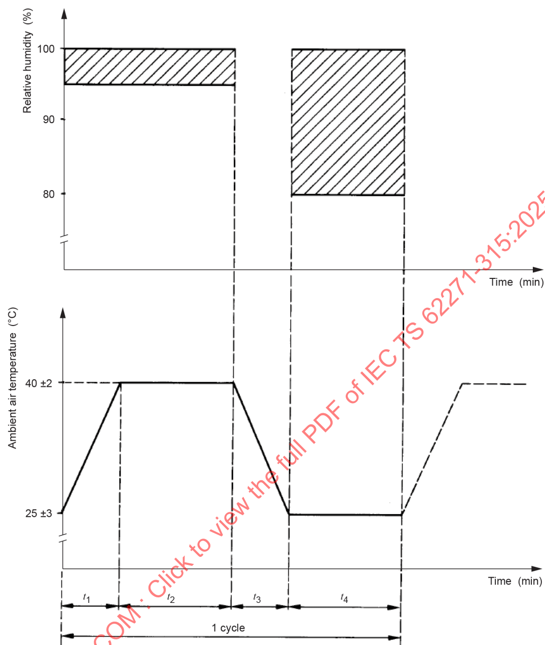
Figure 3 – Humidity test
