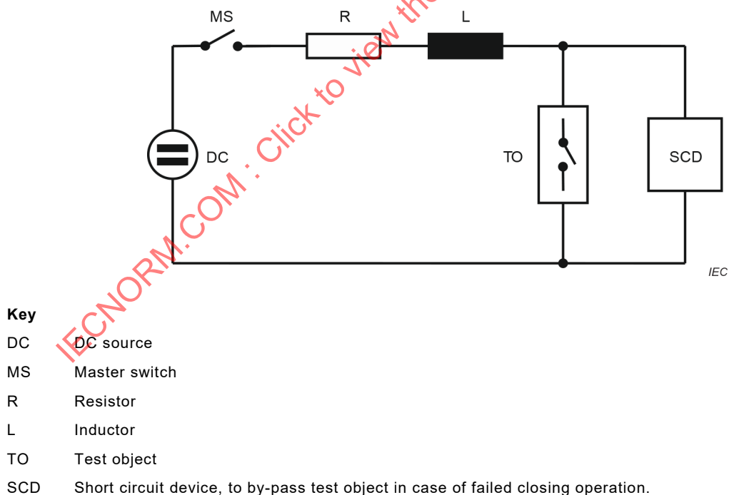
Figure 6 – General layout of test circuit for direct arc withstand test
