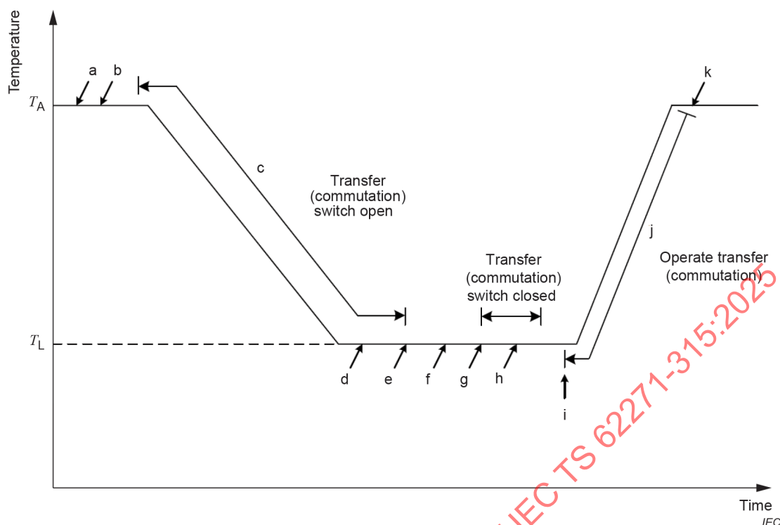
Figure 1 – Test sequence for low temperature test
