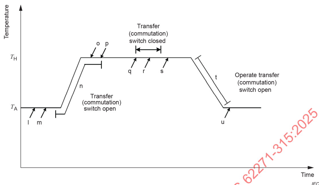
Figure 2 – Test sequence for high temperature test
