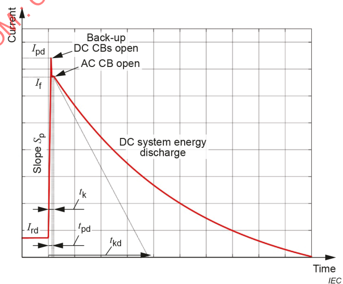
Figure 2 – Typical waveform of a short-circuit current in an HVDC system
