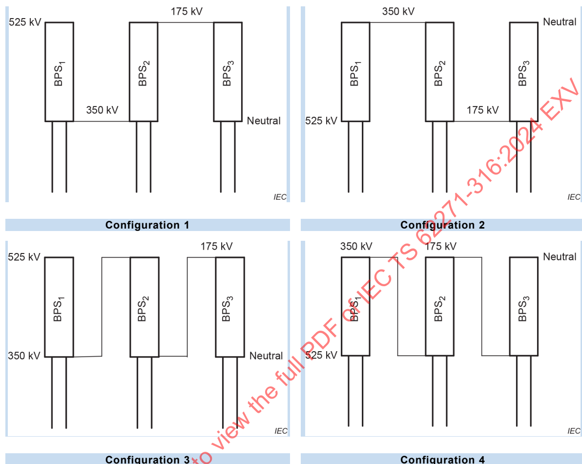
Figure C.2 – Different ways to connect a BPS to the grid
