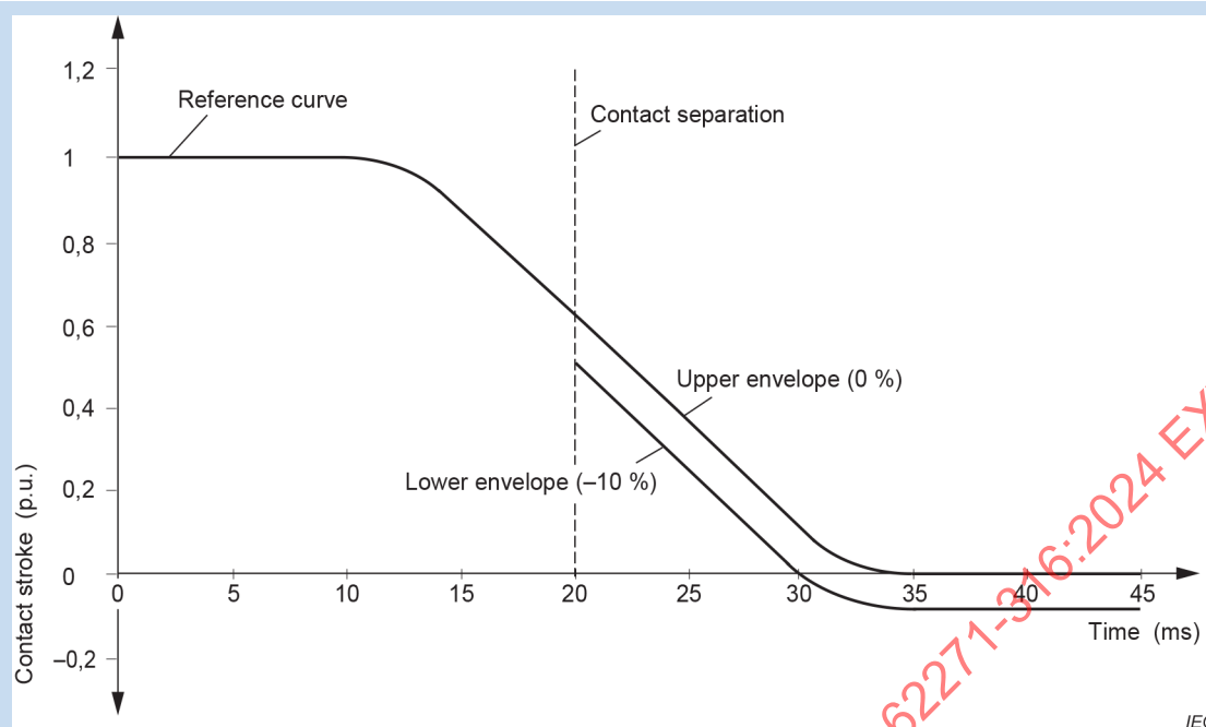
Figure D.4 – Reference mechanical characteristics of Figure D.1 with the envelope fully displaced downward from the reference curve (+0 %, -10 %)
