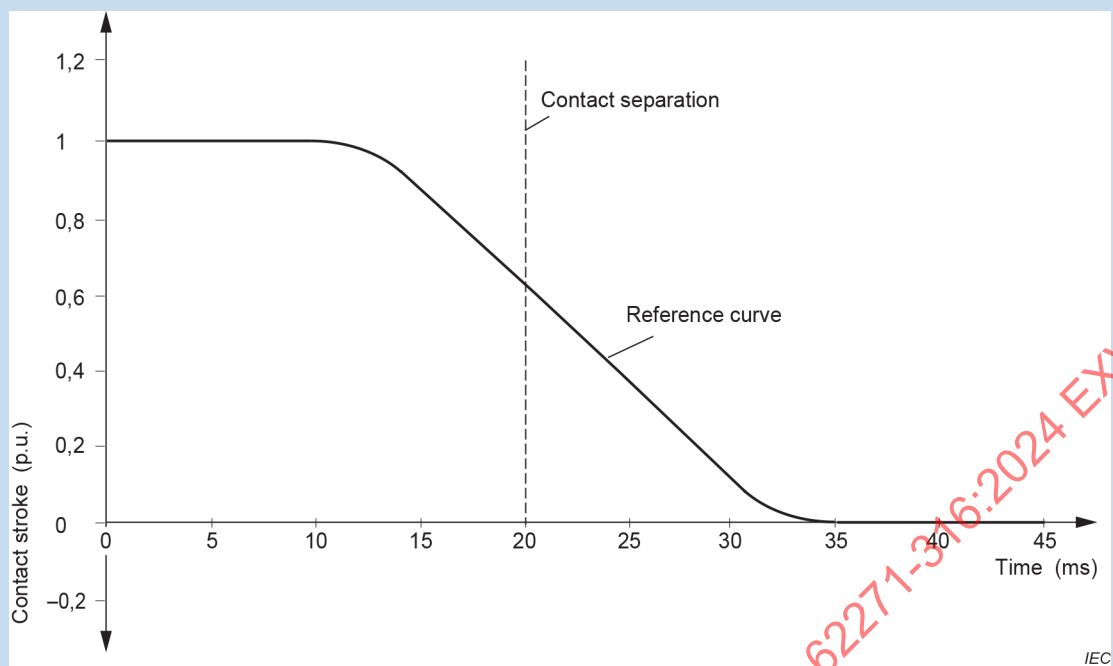
Figure D.1 – Example of reference mechanical characteristics (idealised curve)
