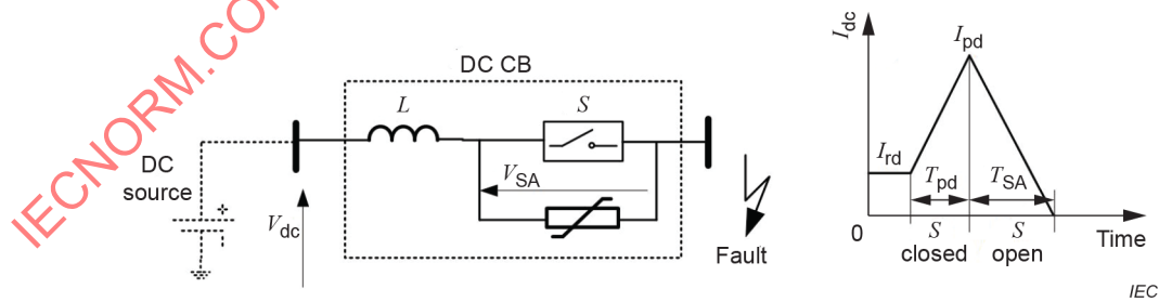
Figure D.5 – DC circuit-breaker simple model
