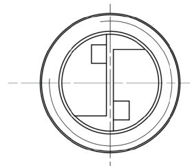
Figure G.2 – Nozzle for weatherproofing test
