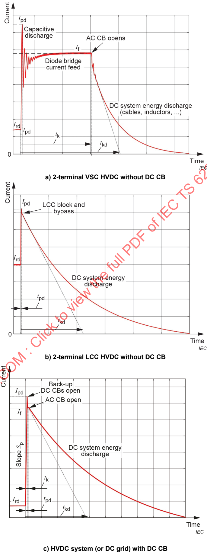
Figure 2 – Typical waveform of a short-circuit current in an HVDC system
