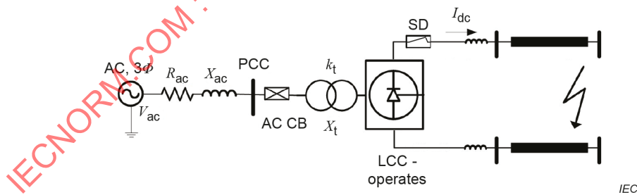
Figure D.2 – LCC HVDC under worst-case, pole-pole DC fault
