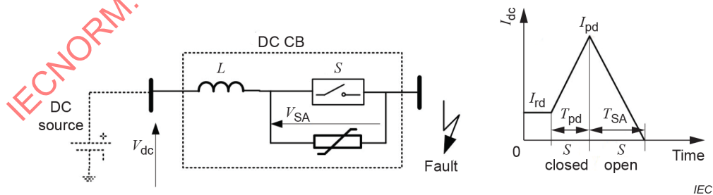
Figure D.5 – DC circuit-breaker simple model
