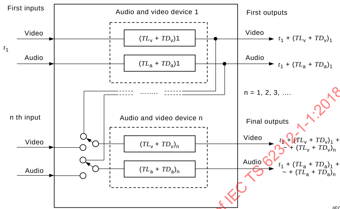
Figure 6 – Compound equipment
