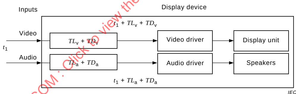
Figure 4 – Display device
