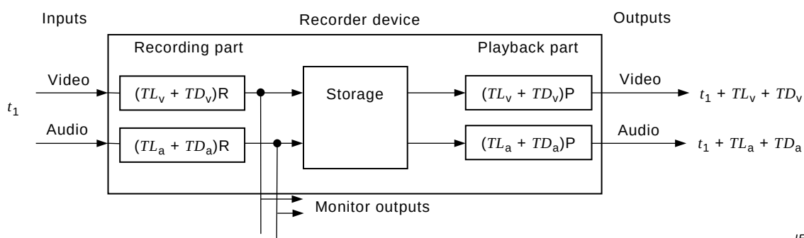
Figure 5 – Recorder device
