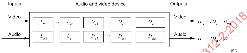
Figure 8 – Additional delay
