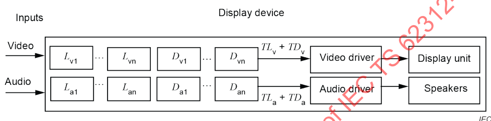
Figure 5 – Display device
