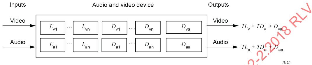
Figure 8 – Additional delay
