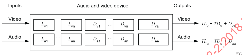
Figure 8 – Additional delay
