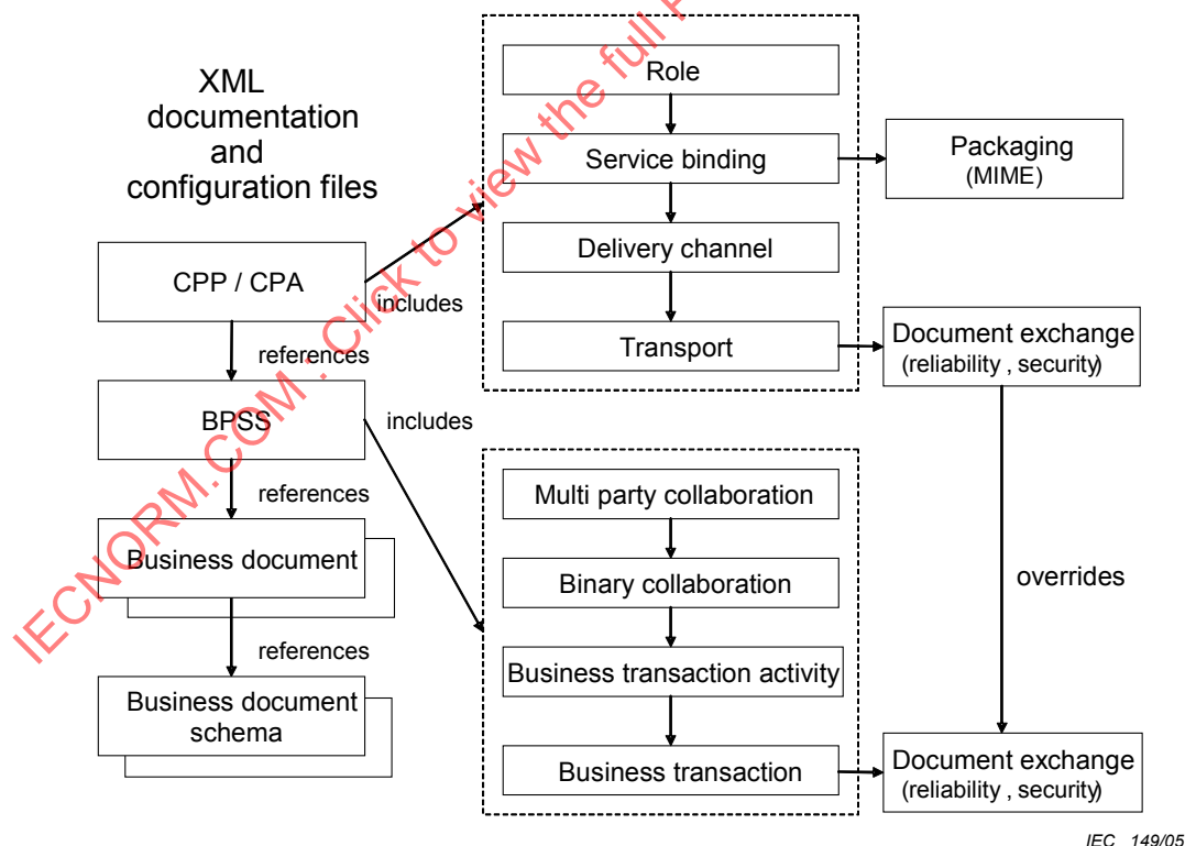
Figure 1 – References and content of ebXML documents
