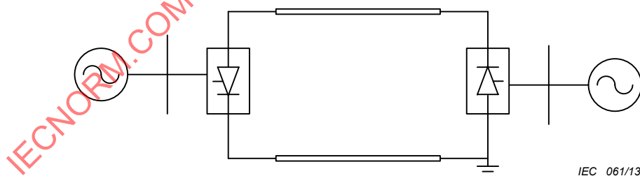
Figure A.3 – Schematic diagram of the structure of monopolar metallic return system
