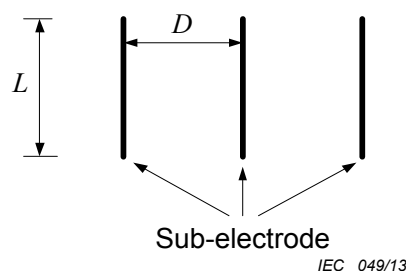
Figure 2 – Vertical arrangement
