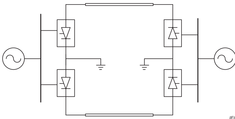
Figure A.4 – Schematic diagram of bipolar earth/sea water system
