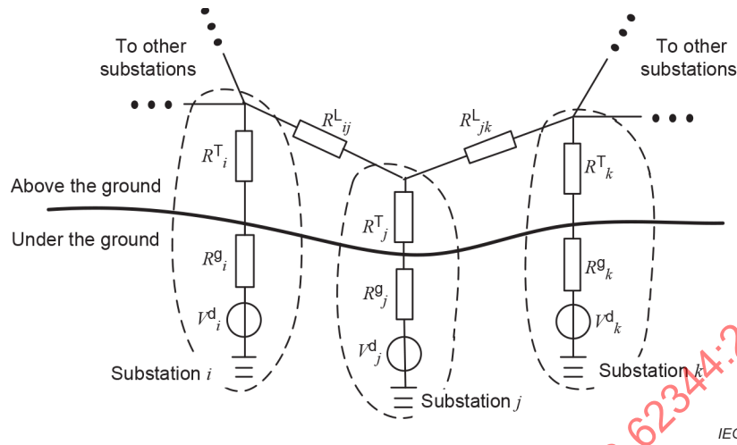
Figure K.2 – Circuit model for the analysis of DC distribution of AC systems
