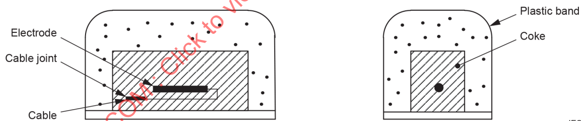
Figure 5 – Sea electrode
