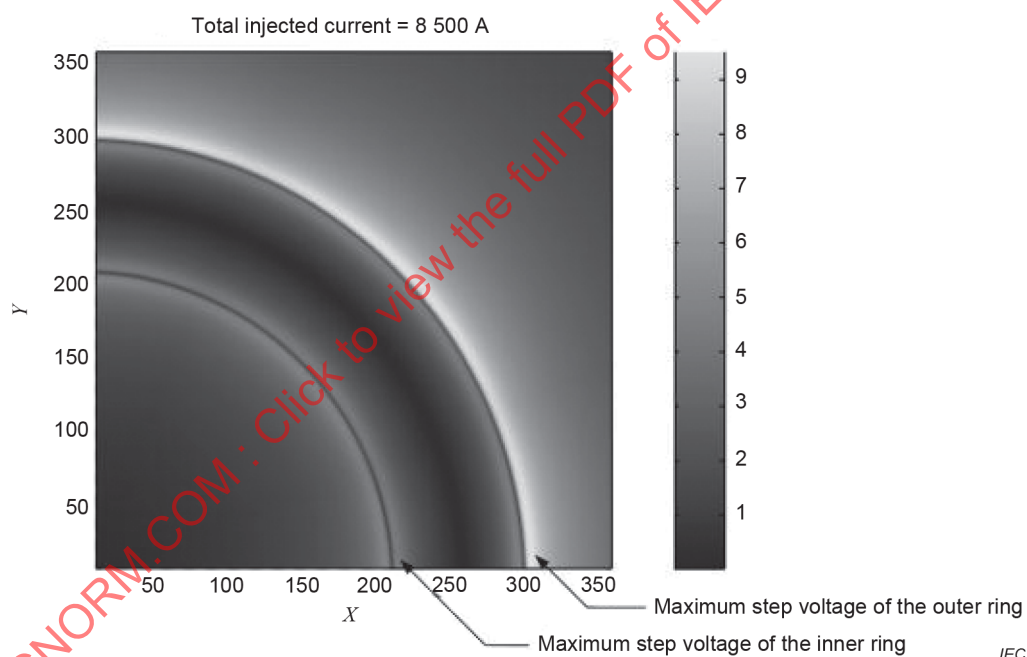
Figure G.9 – Ground potential and step voltage distribution of a double-circle earth electrode
