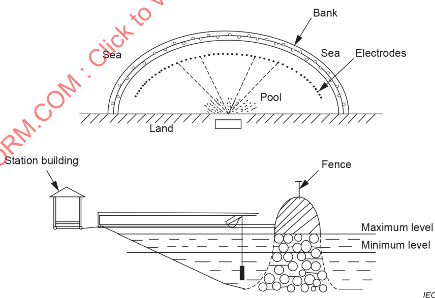
Figure M.2 – Shore electrode, pond type
