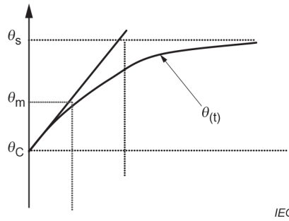
Figure H.1 – Earth electrode temperature rise characteristics
