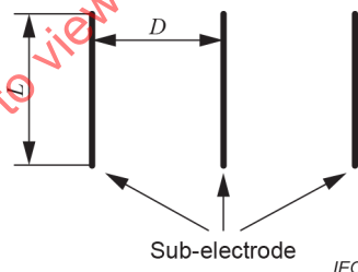
Figure 2 – Vertical arrangement
