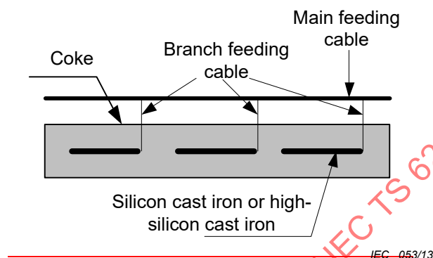
b) Silicon cast iron or high-silicon cast iron used for feeding rod
