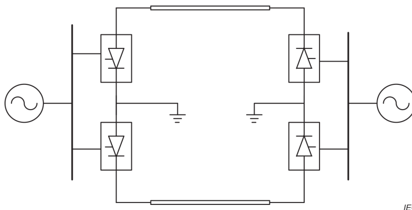
Figure A.4 – Schematic diagram of the structure of bipolar neutral grounded at both ends bipolar earth/sea water system
