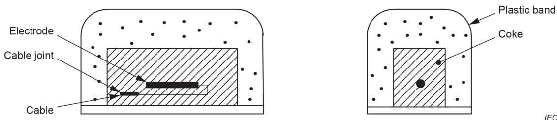
Figure 5 – Sea electrode
