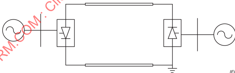
Figure A.3 – Schematic diagram of the structure of monopolar dedicated metallic return system
