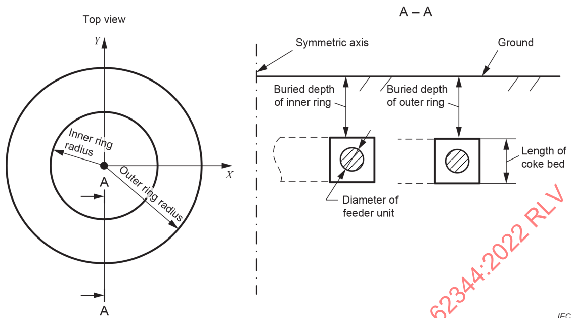
Figure G.8 – Structure of a double-circle DC earth electrode
