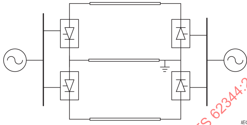
Figure A.6 – Schematic diagram of the structure of bipolar neutral line bipolar dedicated metallic return system
