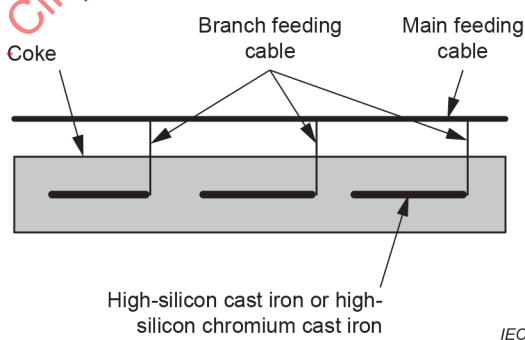
b) High-silicon cast iron or high-silicon chromium cast iron used for electrode element
