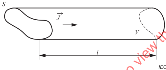
Figure G.2 – Ohm's law applied to cylinder conductor
