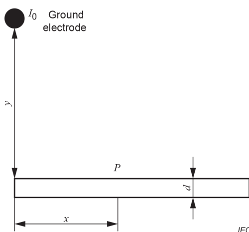
Figure J.1 – Calculation of current flowing through a metal pipe
