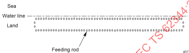
Figure M.1 – Top view of shore electrode, beach type
