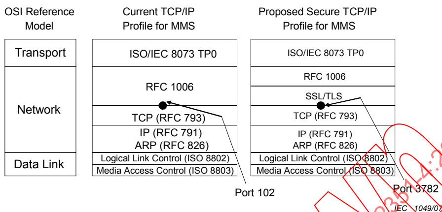
Figure 2 – Non-secure and secure TCP T-Profiles IEC 62351
