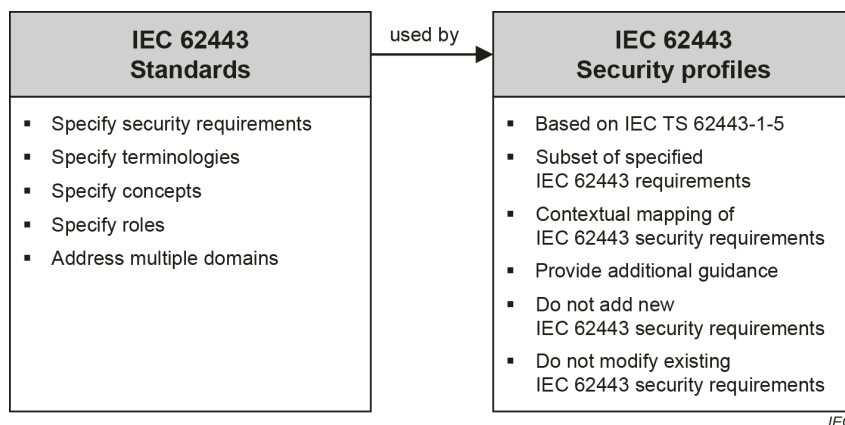
Figure 1 – Relationship between standards and security profiles within the IEC 62443 series
