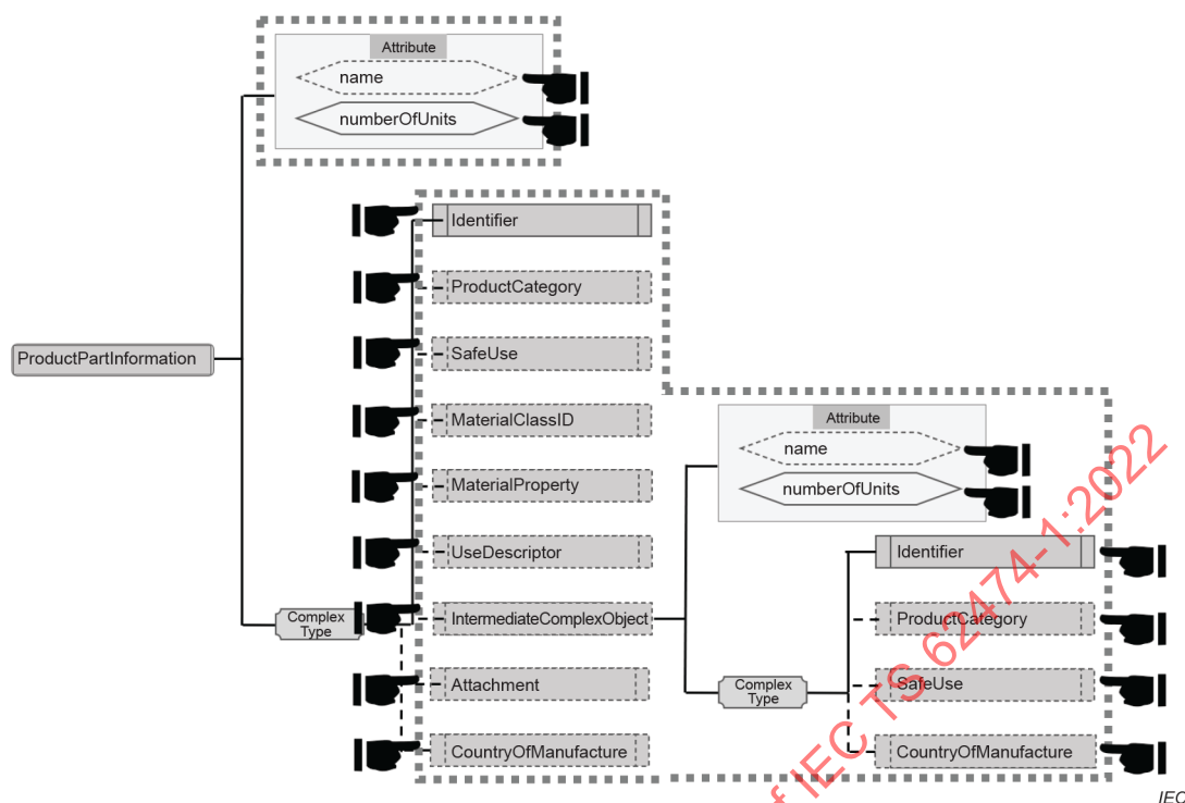
Figure 8 – ProductPartInformation element for the declarable articles
