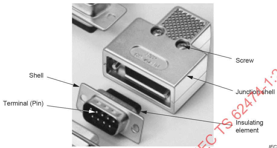
Figure 12 – Product – Connector
