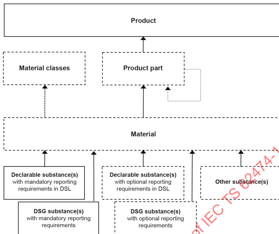
Figure 15 – Data model for a composition declaration
