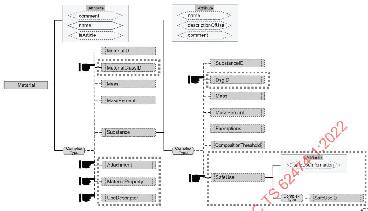
Figure 9 – Material element supporting SCIP information
