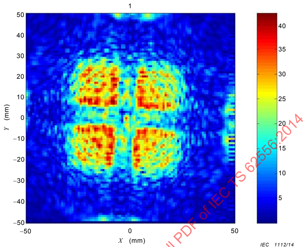
Figure F.2 – Pressure amplitude as scanned
