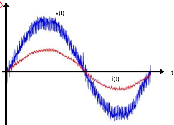
Figure 8 – Typical mains current and voltage of an AIC realized by a PWM Converter with capacitive smoothing without additional filters
